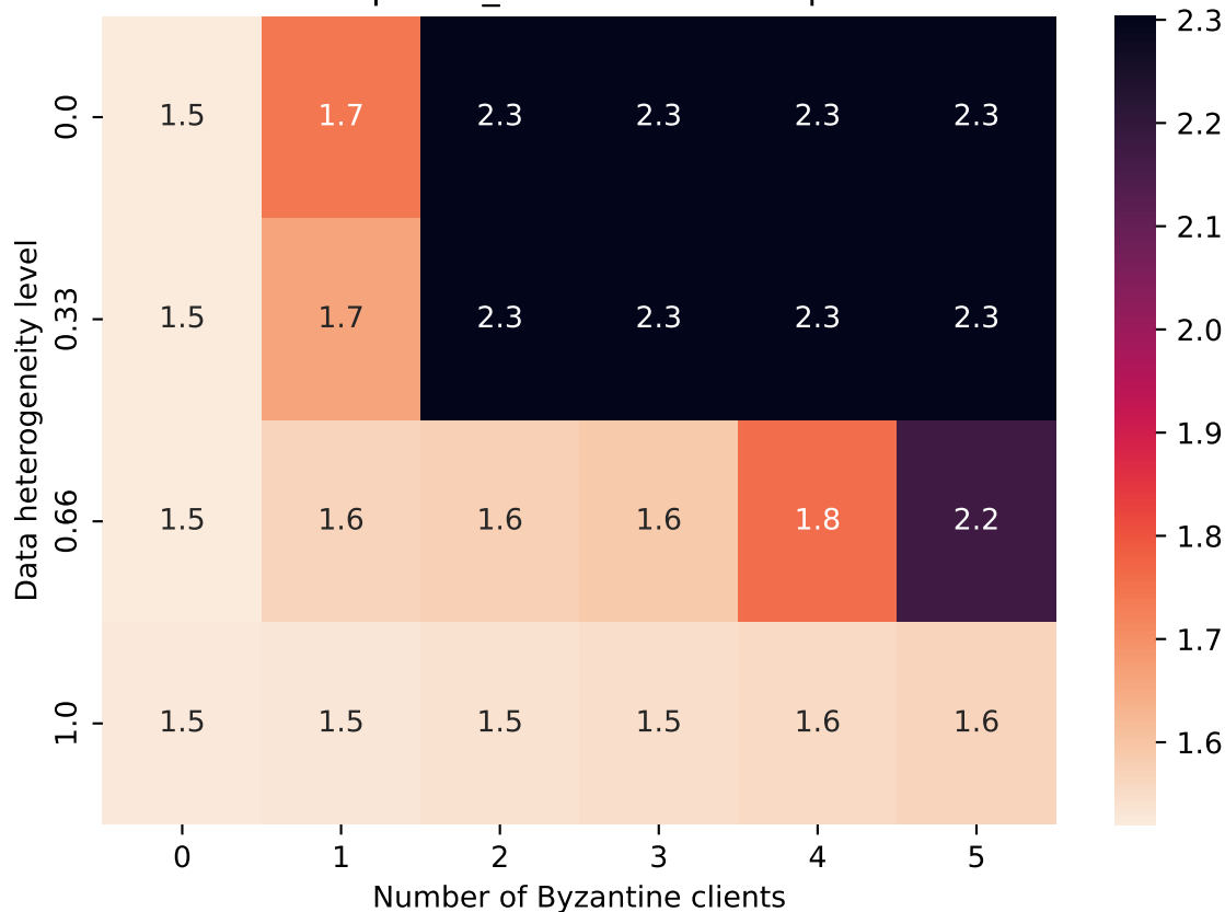
Attack: Optimal_InnerProductManipulation
