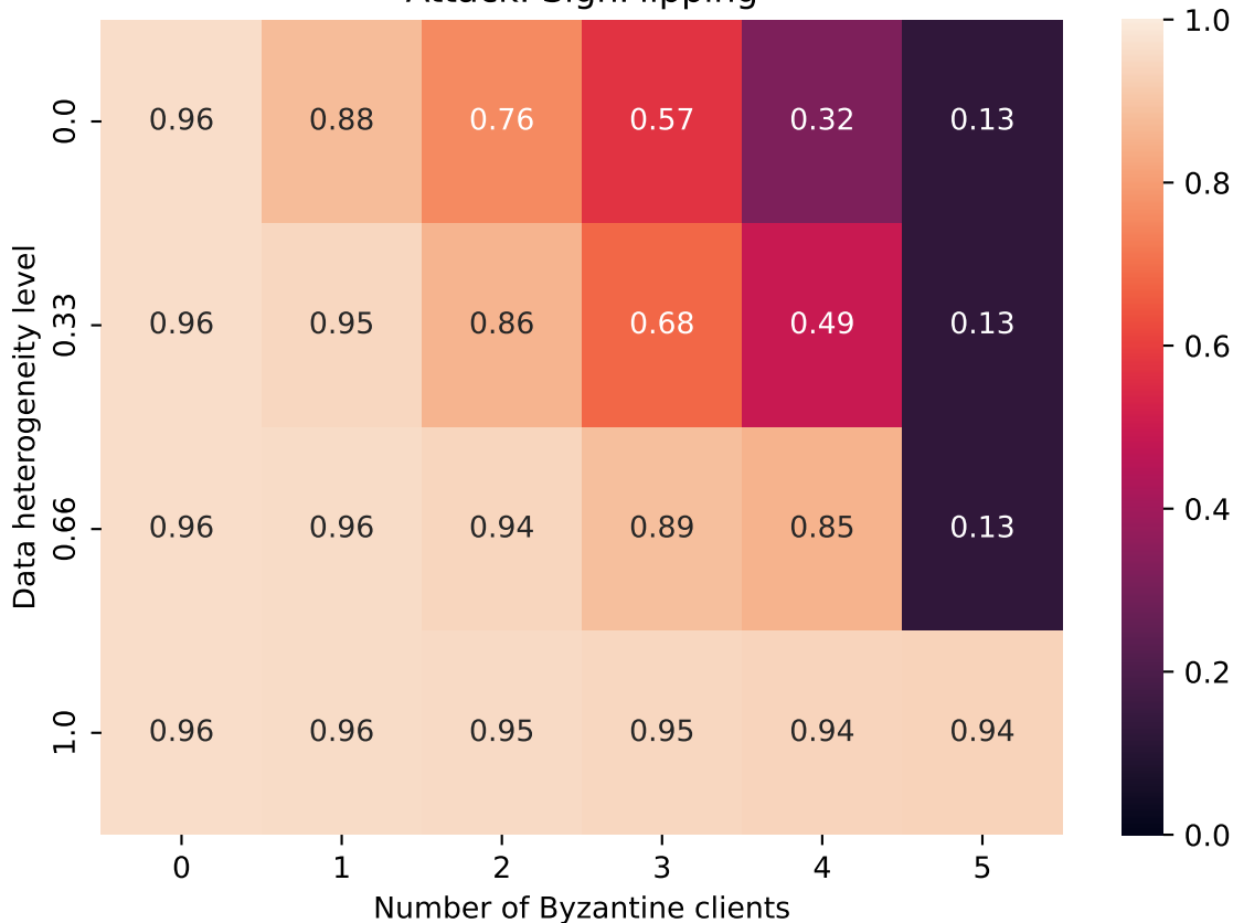
Attack: SignFlipping
