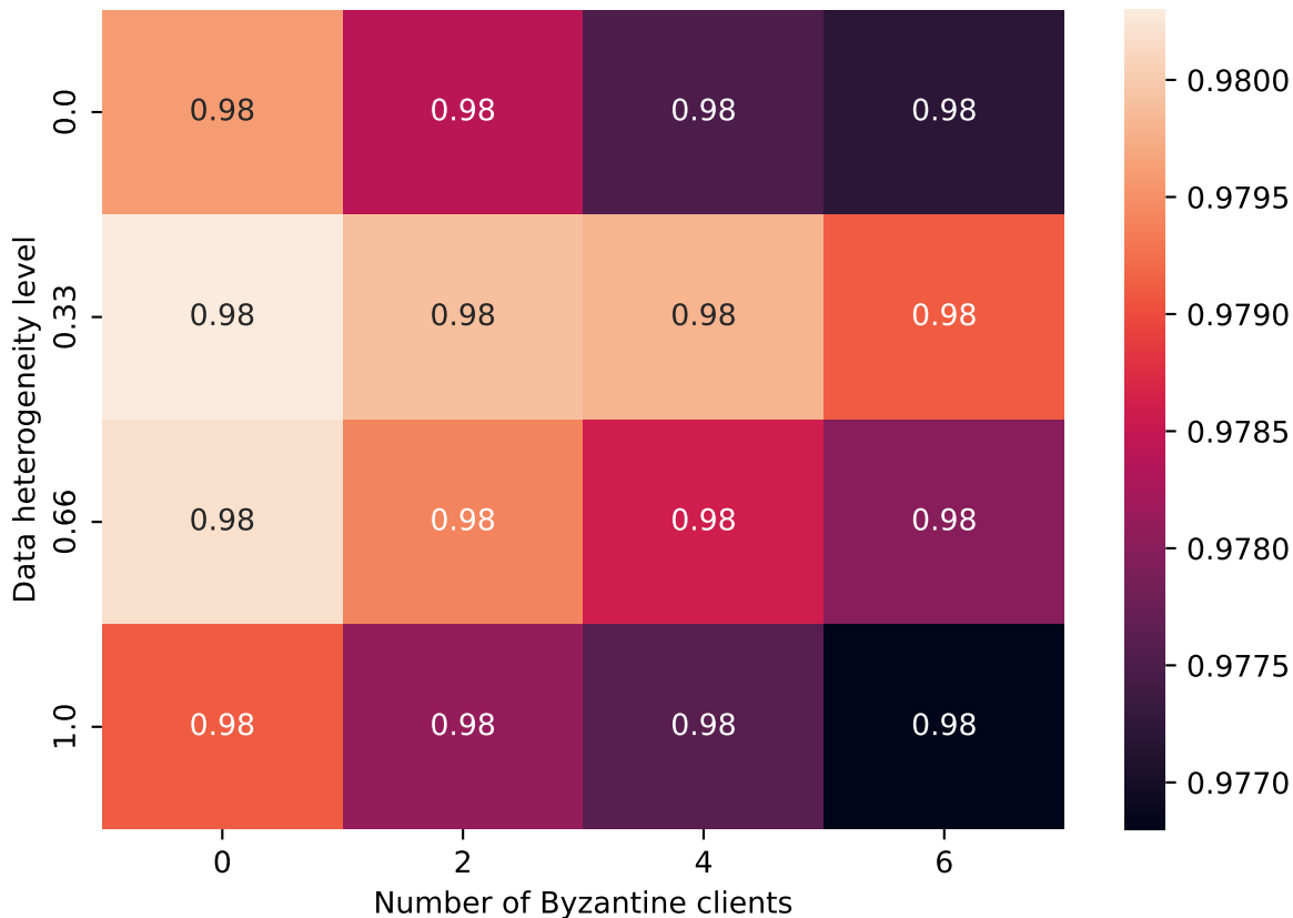
Attack: Gaussian
