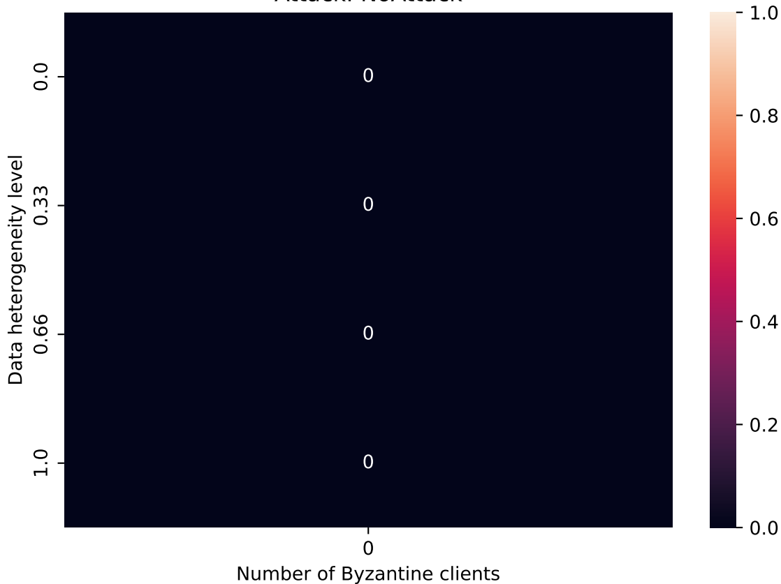
Attack: NoAttack
