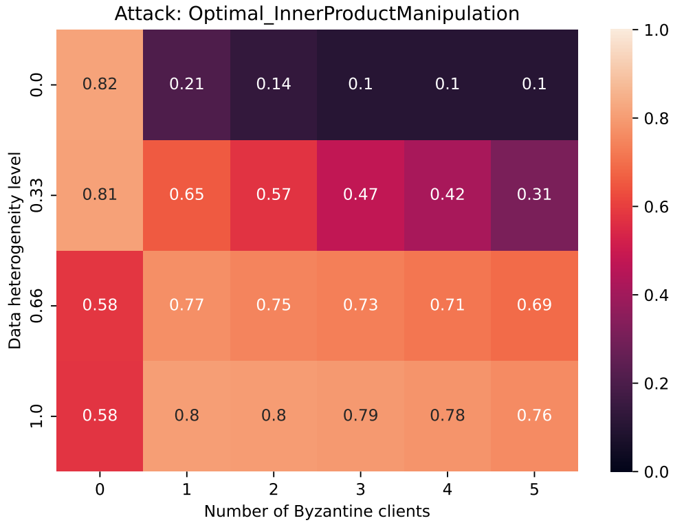
Figure 4: Best test accuracy under OptIPM.
