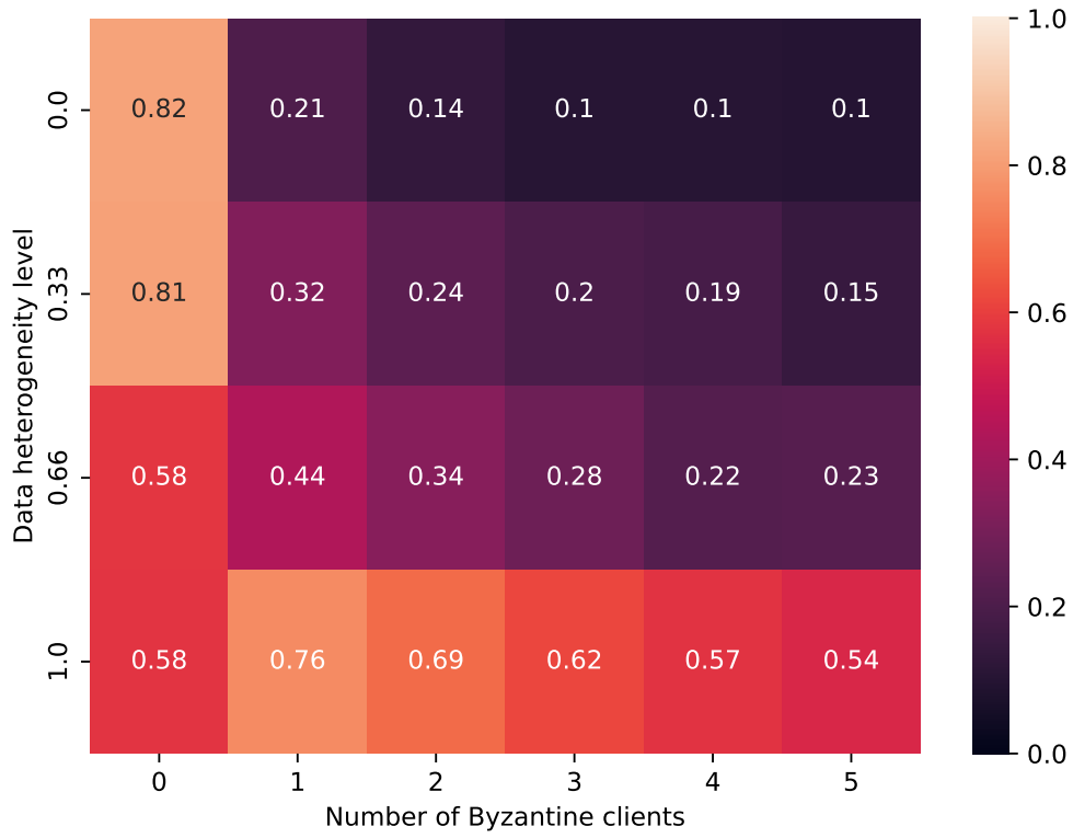
Figure 1: Best overall test accuracy (worst-case across attacks).
