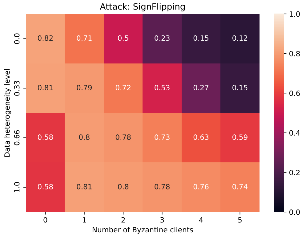
Figure 3: Best test accuracy under Sign Flipping.
