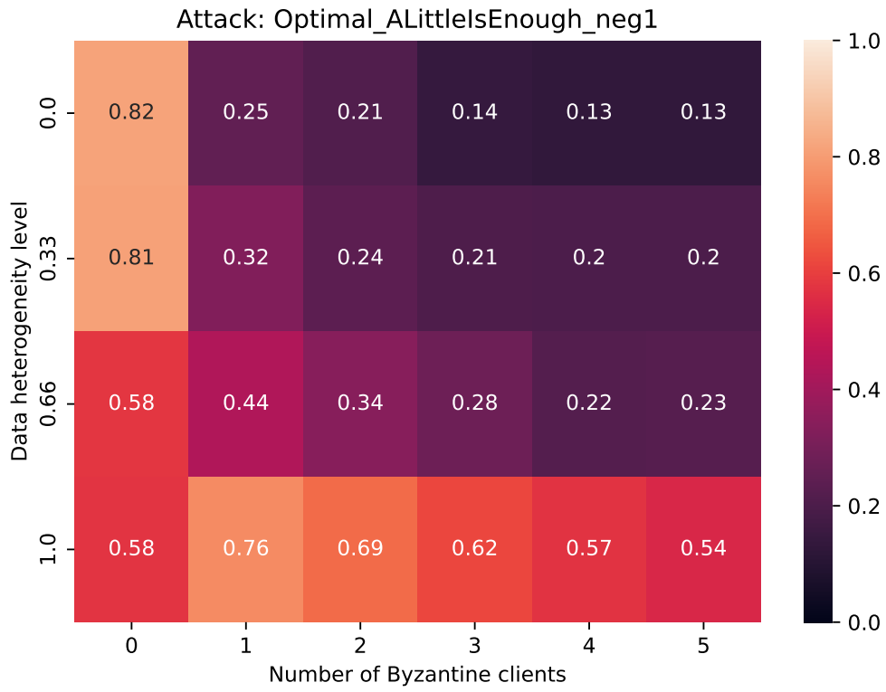
Figure 2: Best test accuracy under OptALIE.
