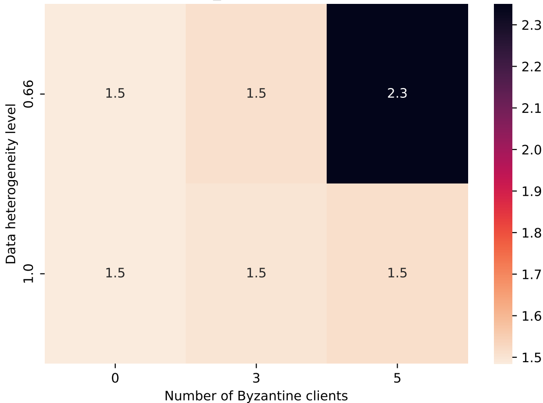
Attack: Optimal_InnerProductManipulation
