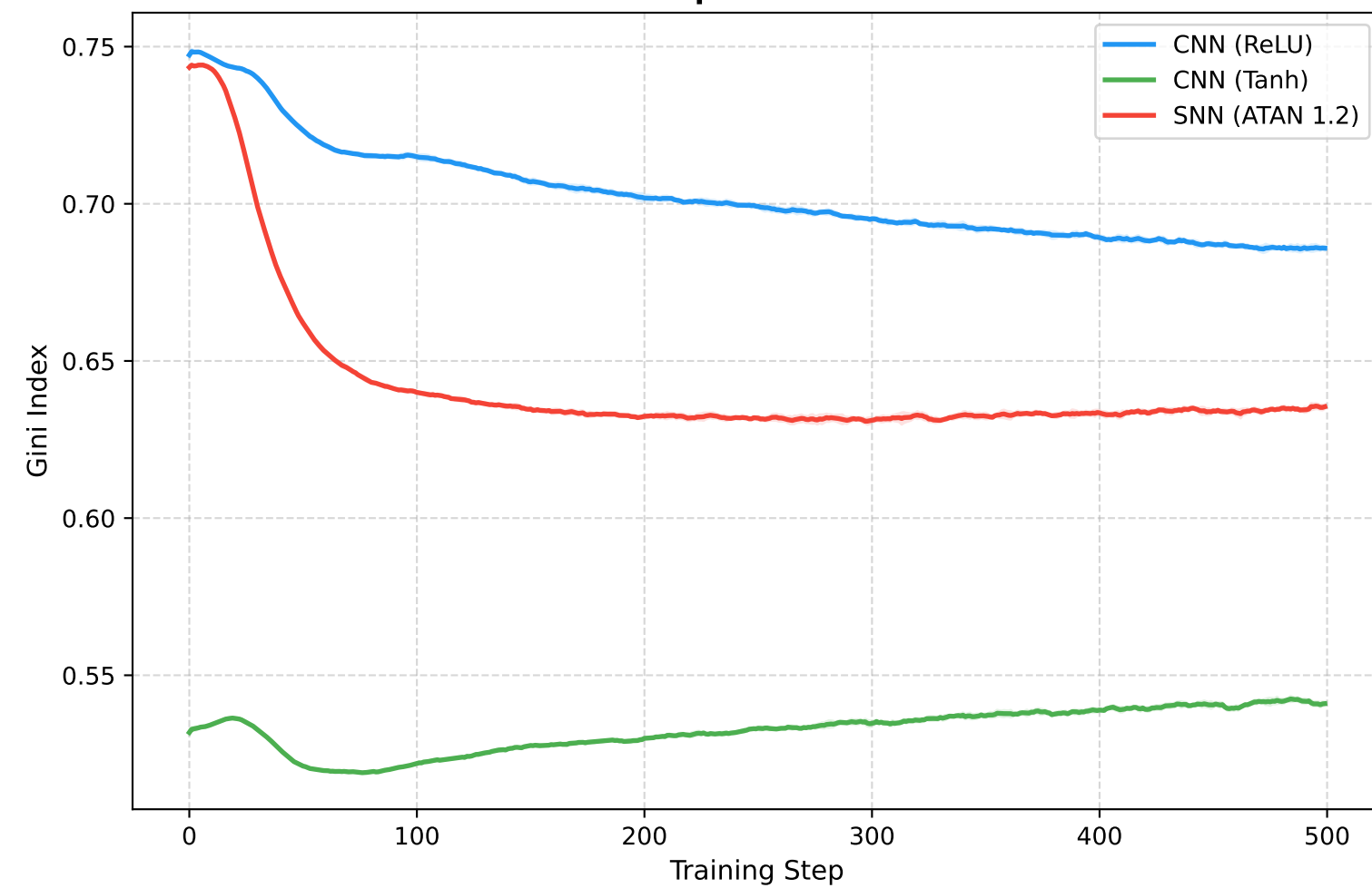
\gamma = 0.33
