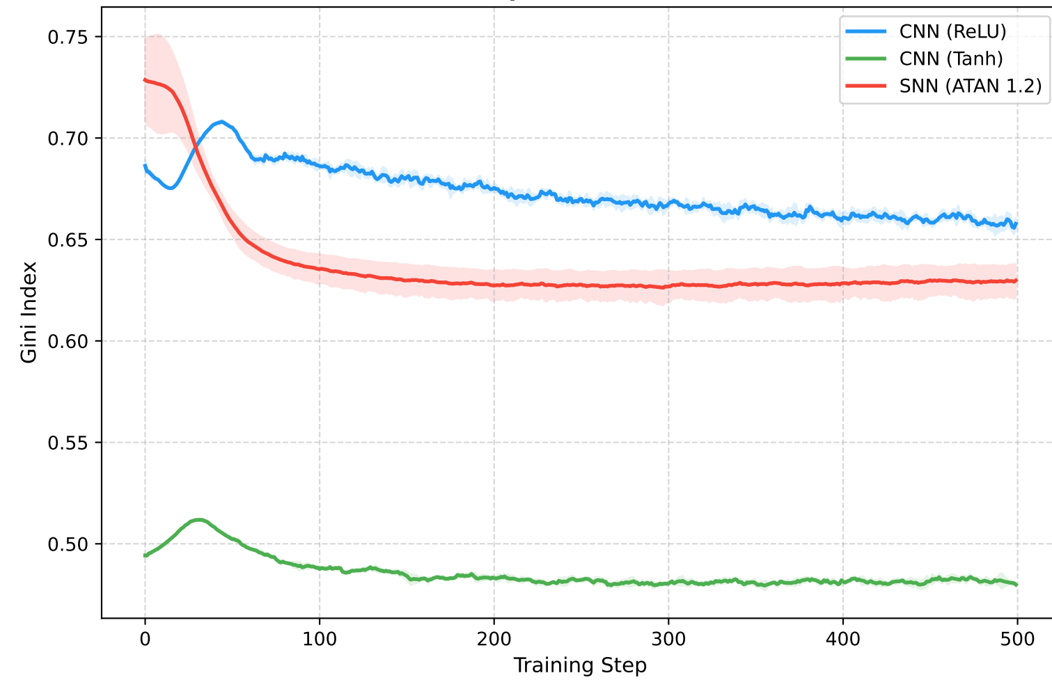
\gamma = 0.33
