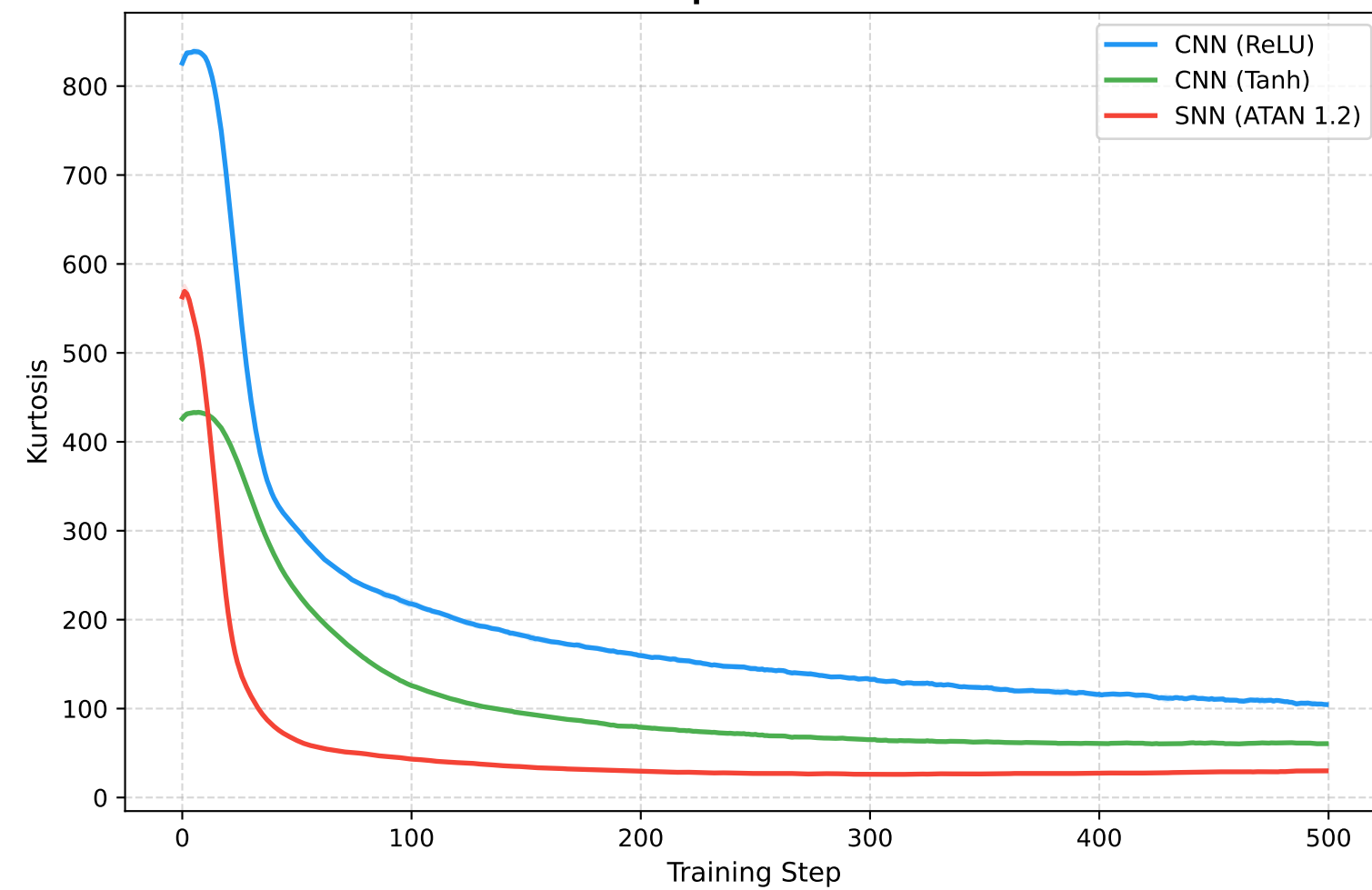
\gamma = 0.33
