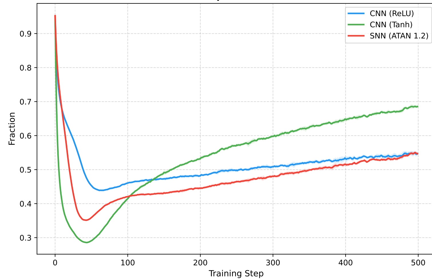
\gamma = 0.33
