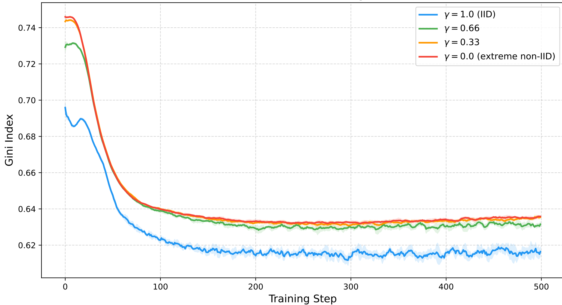
Gini Index (SNN ATAN \alpha=1.2 , f=0 , Average, n=10 )
