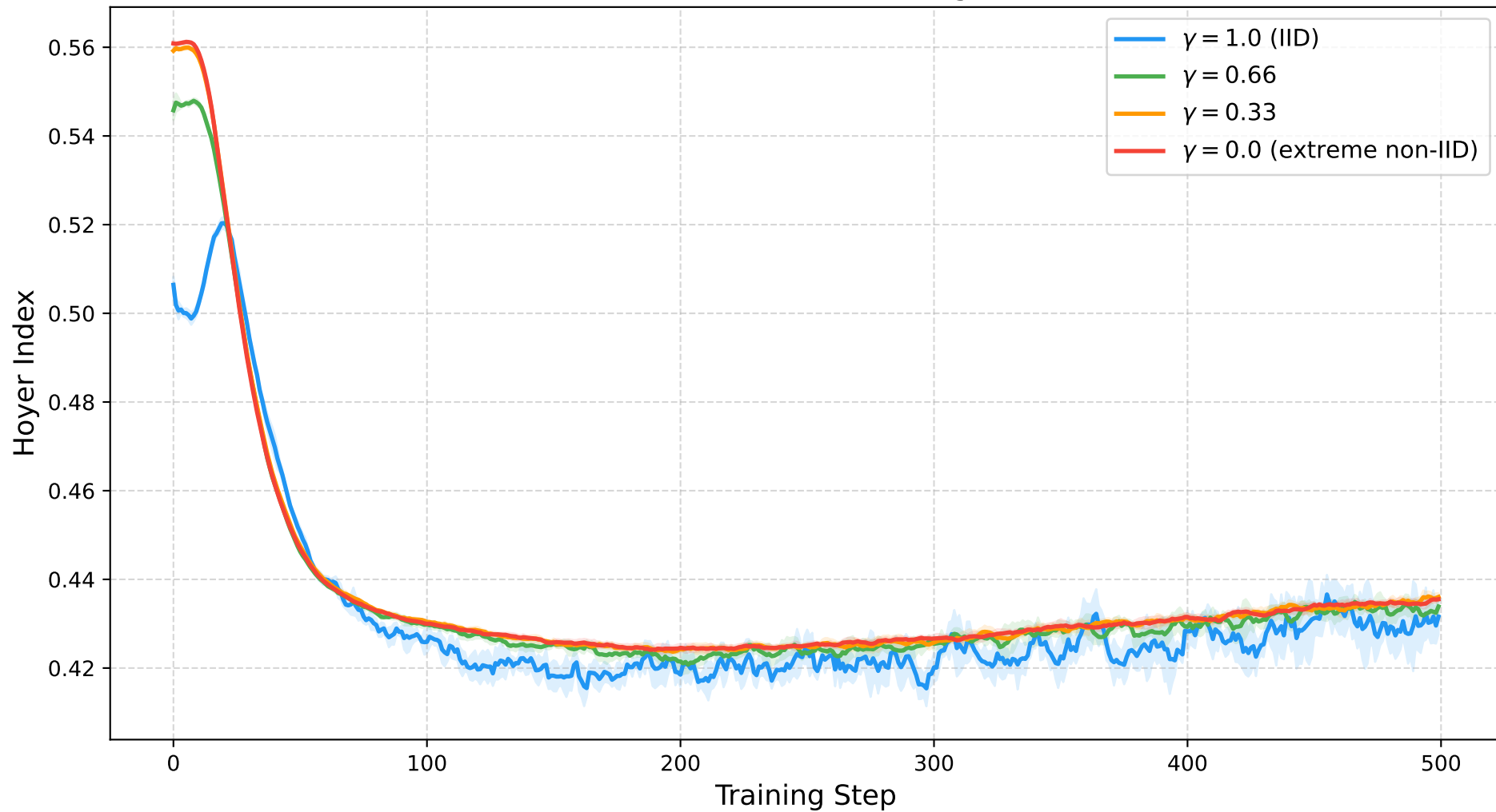
Hoyer Sparsity (SNN ATAN \alpha=1.2 , f=0 , Average, n=10 )
