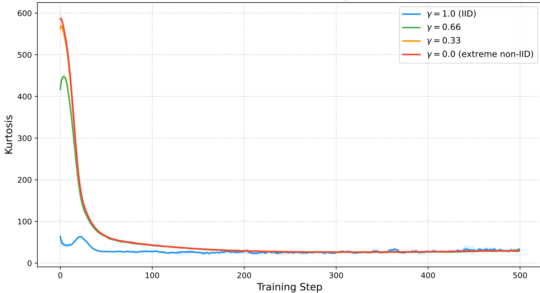
Excess Kurtosis (SNN ATAN \alpha=1.2 , f=0 , Average, n=10 )
