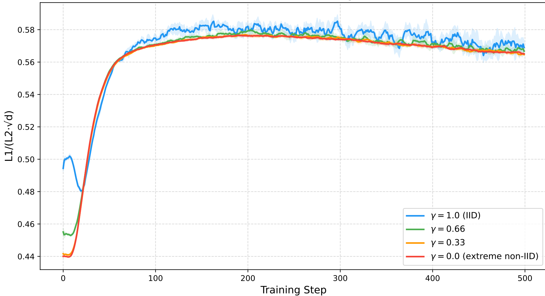
Normalized L1/L2 Ratio (SNN ATAN \alpha=1.2 , f=0 , Average, n=10 )
