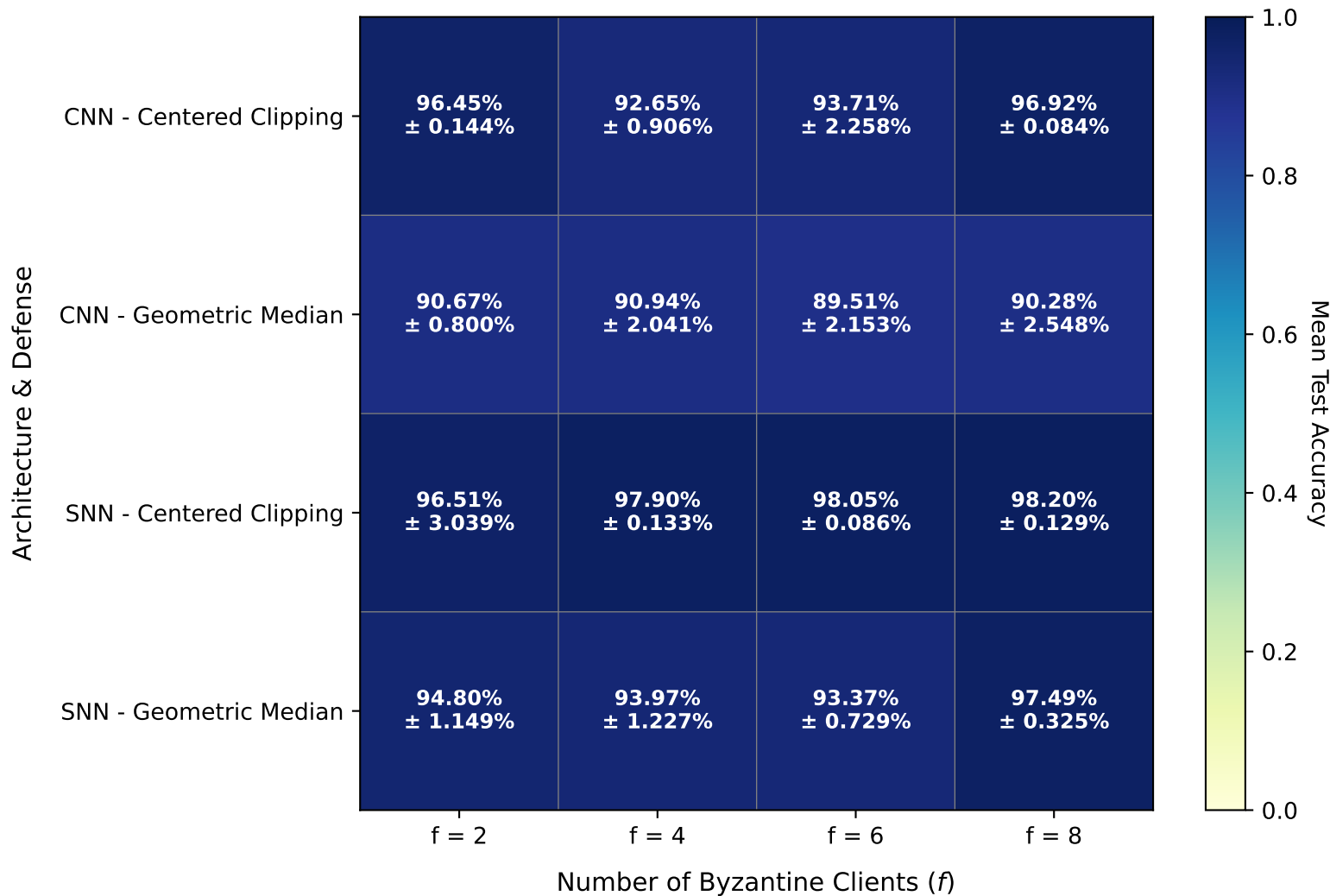
Mean Accuracy Under Optimal A Little Is Enough (ALIE) (Seeds 42-46)
