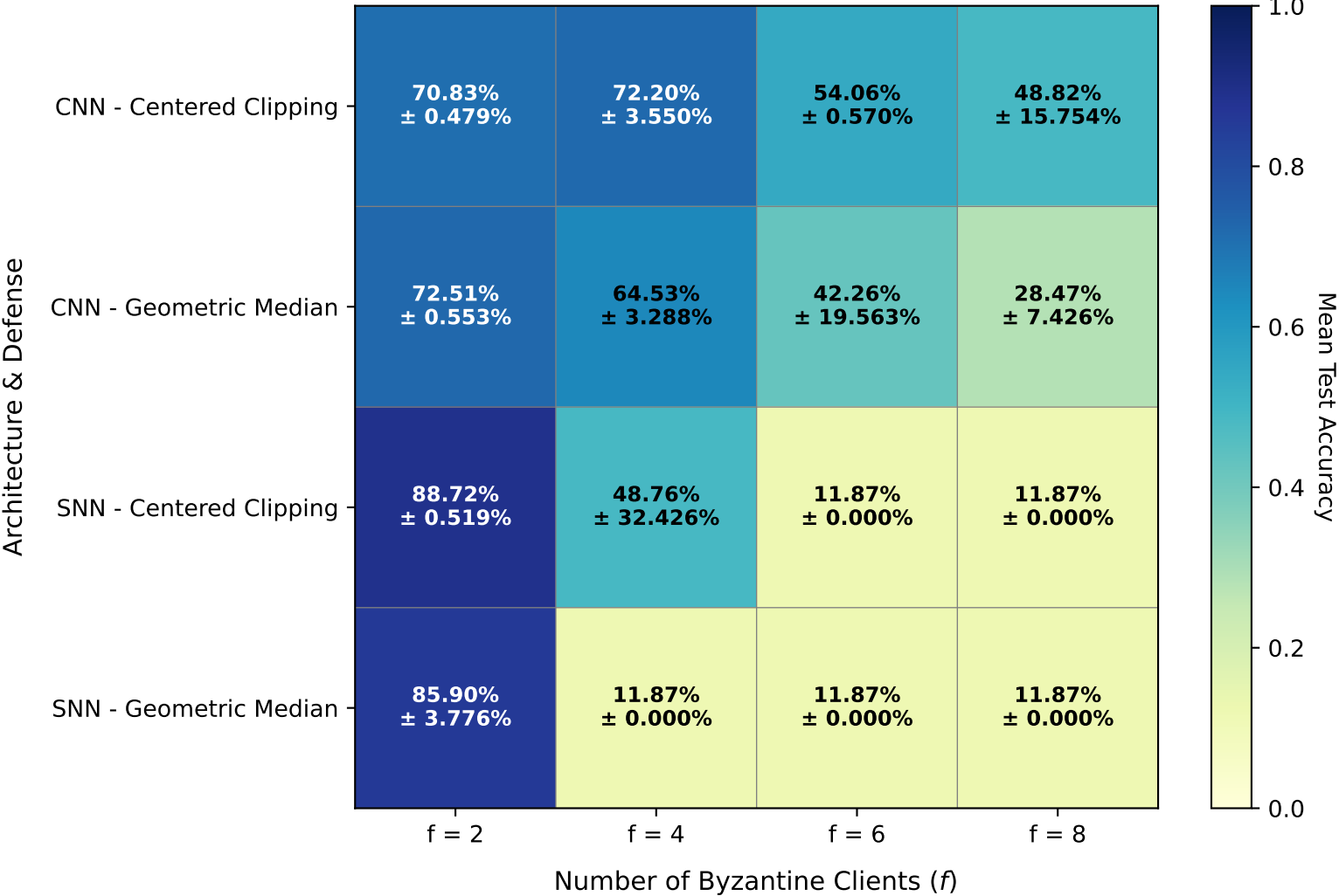
Mean Accuracy Under Optimal Inner Product Manipulation (IPM) (Seeds 42-46)
