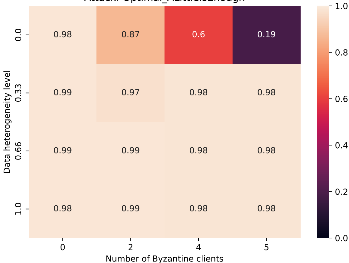
Attack: Optimal_ALittleIsEnough
