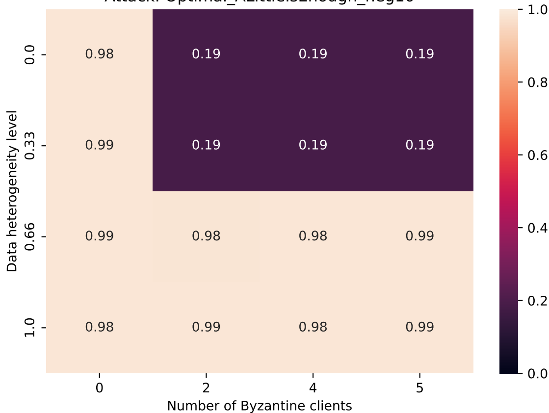
Attack: Optimal_ALittleIsEnough_neg10
