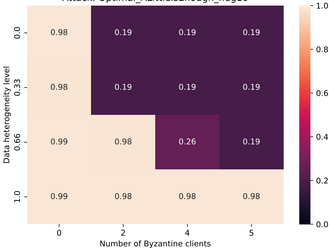
Attack: Optimal_ALittleIsEnough_neg10
