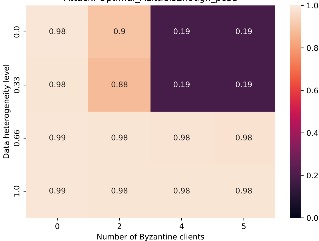
Attack: Optimal_ALittleIsEnough_pos1
