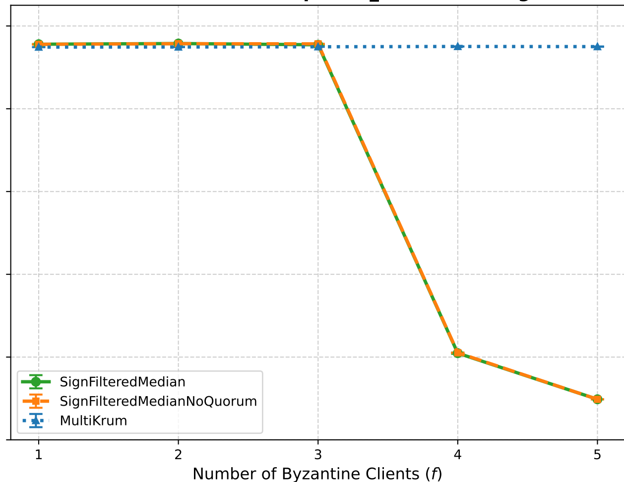
Robustness under Optimal_ALittleIsEnough
