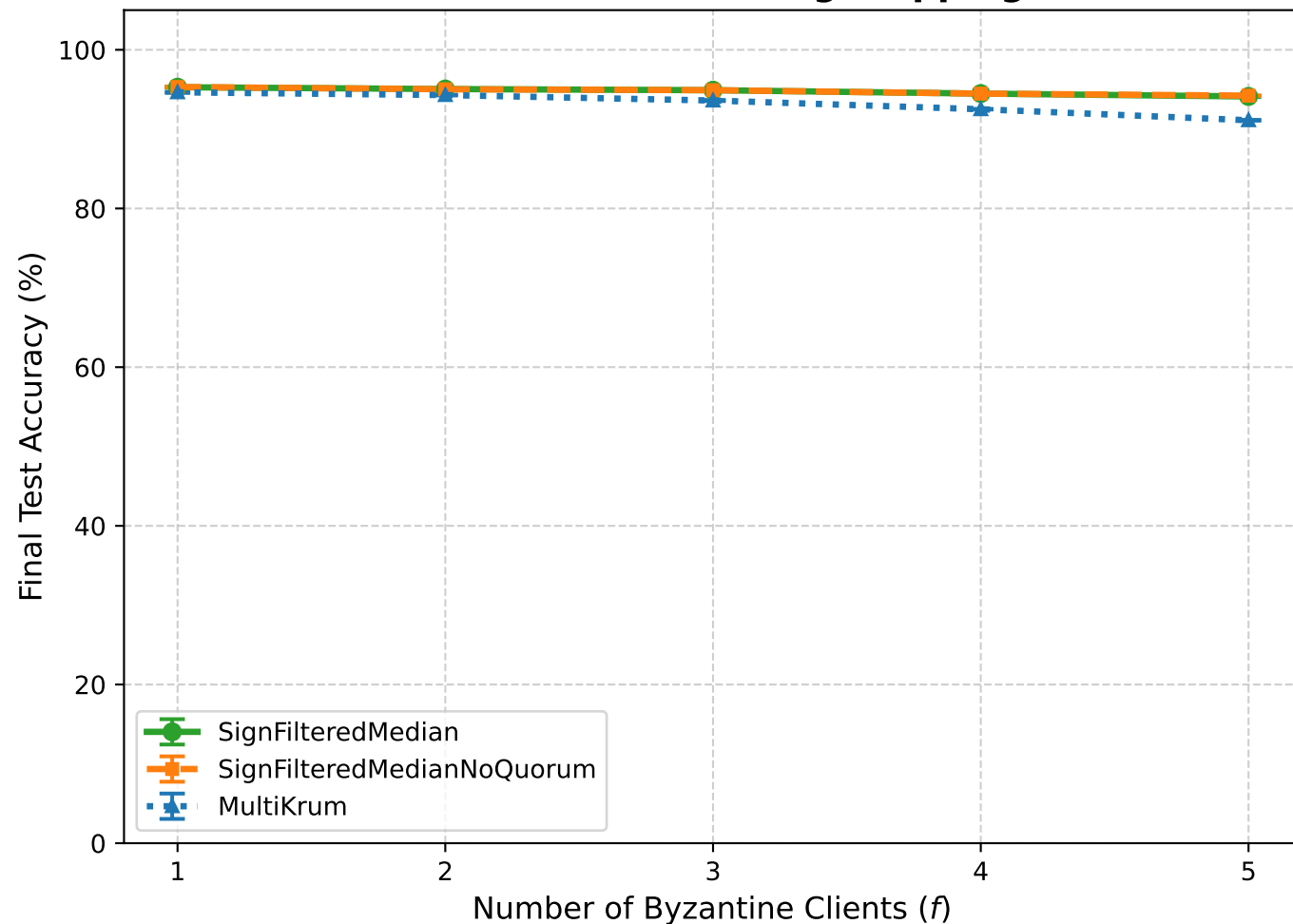
Robustness under SignFlipping
