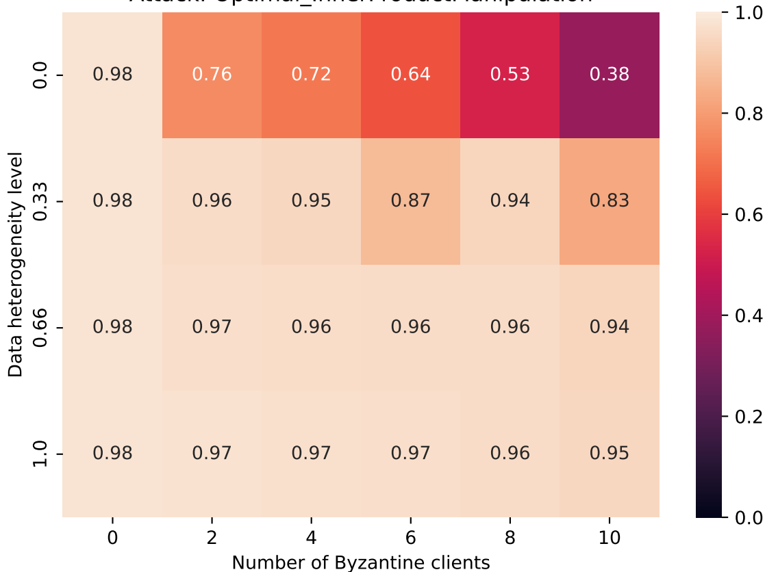
Attack: Optimal_InnerProductManipulation
