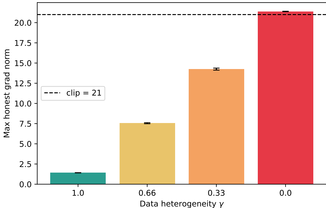
SNN max honest gradient norm vs heterogeneity (no attack)
