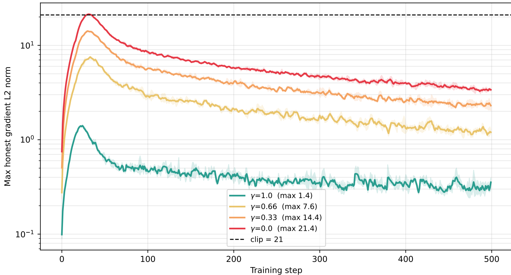
SNN (atan \alpha=1.2 , \beta=0.95 , T=10 ) — max honest gradient norm, no attack
