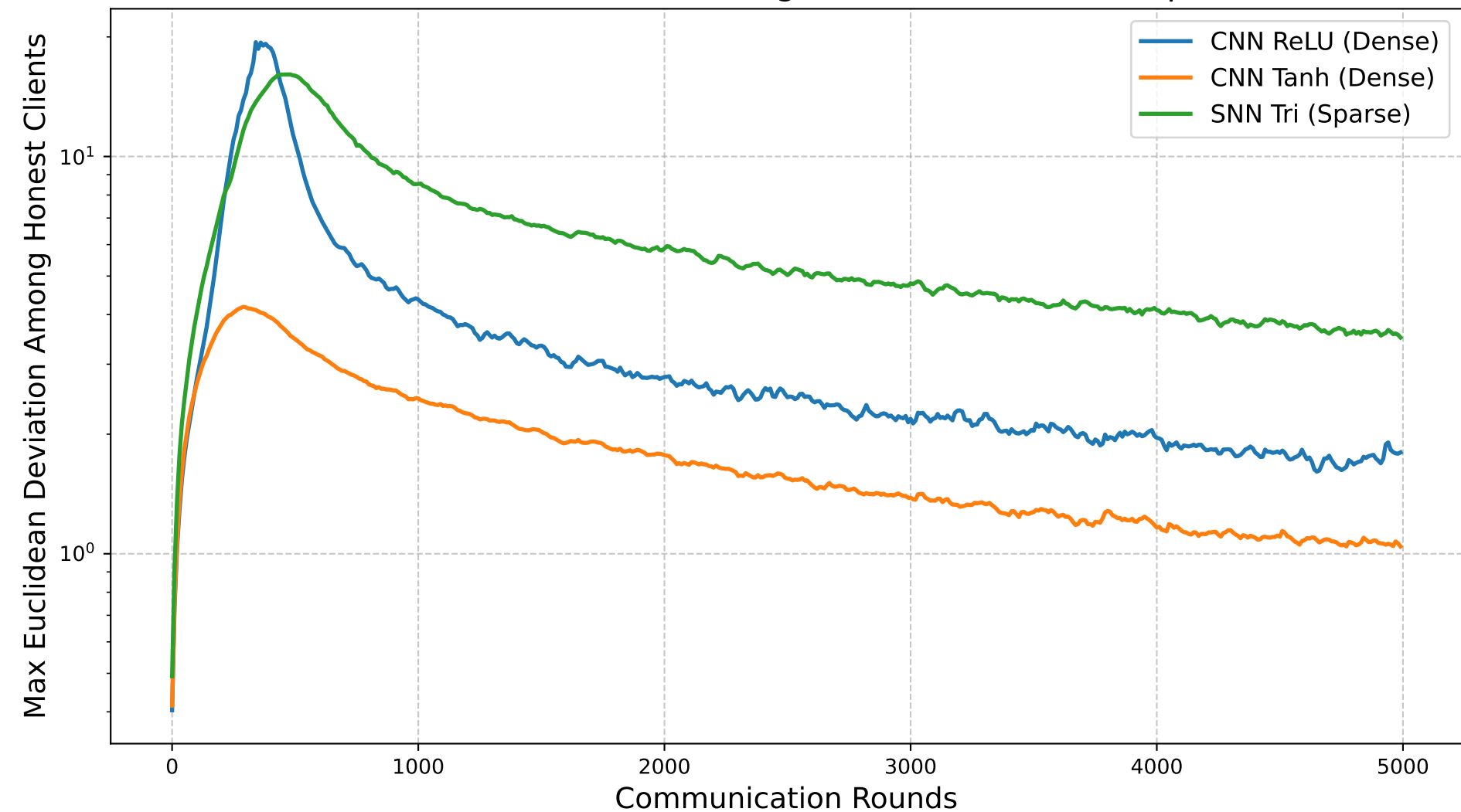
Max Euclidean Deviation Among Honest Clients ( f = 0 , \gamma = 0.33 )
