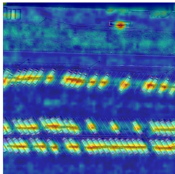
(b) RTMDet
