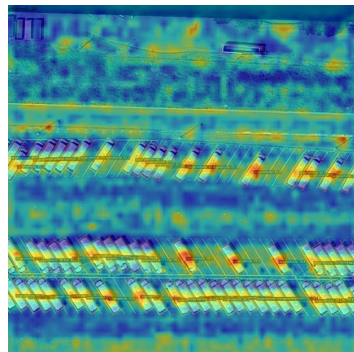
(c) YOLOMS
