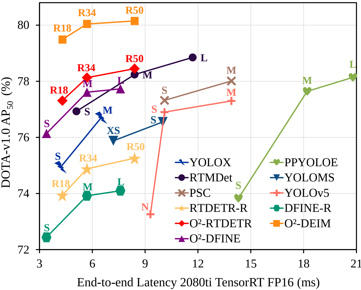
Oriented Object Detection on DOTA-v1.0
