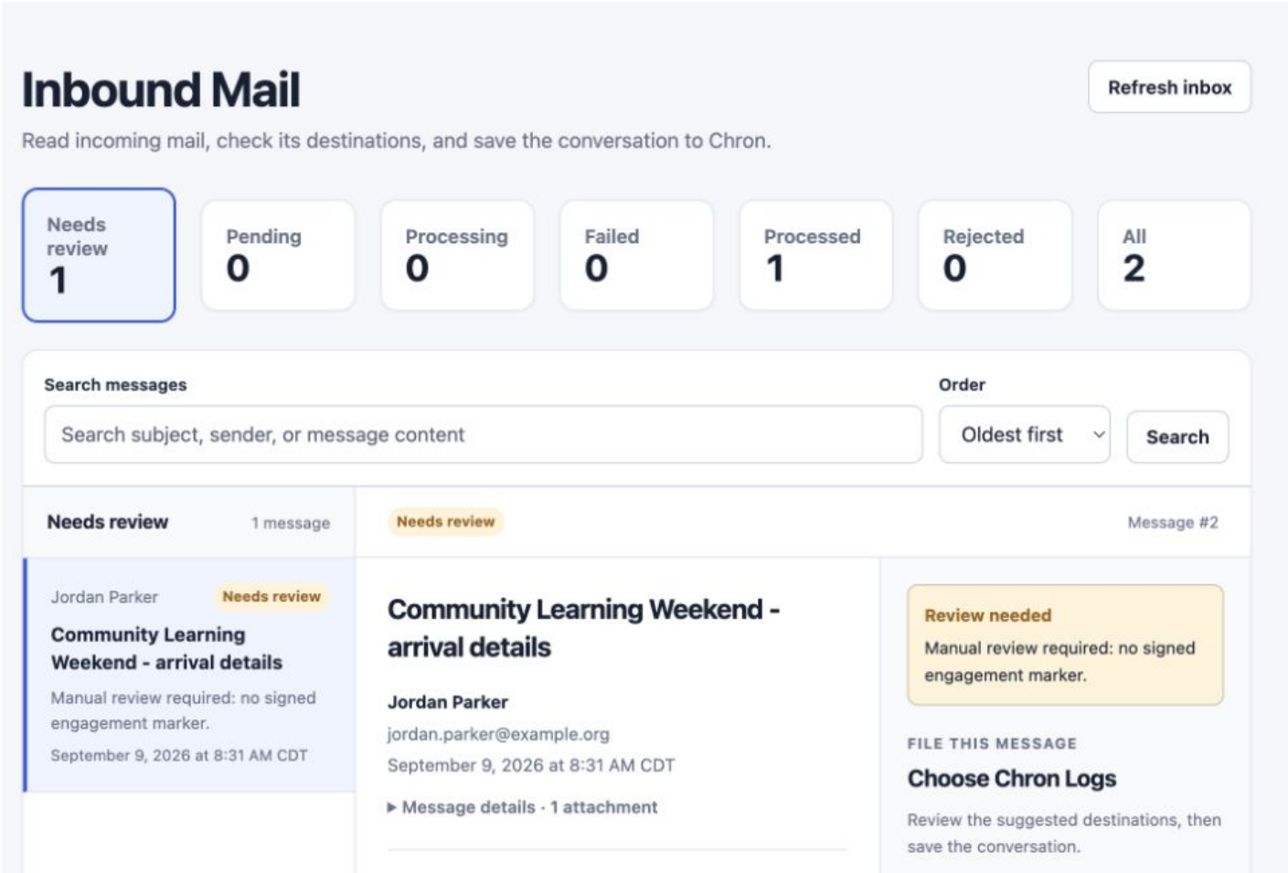
Figure 54. Review copied inbound email. Actual preview screen; fictional records.
