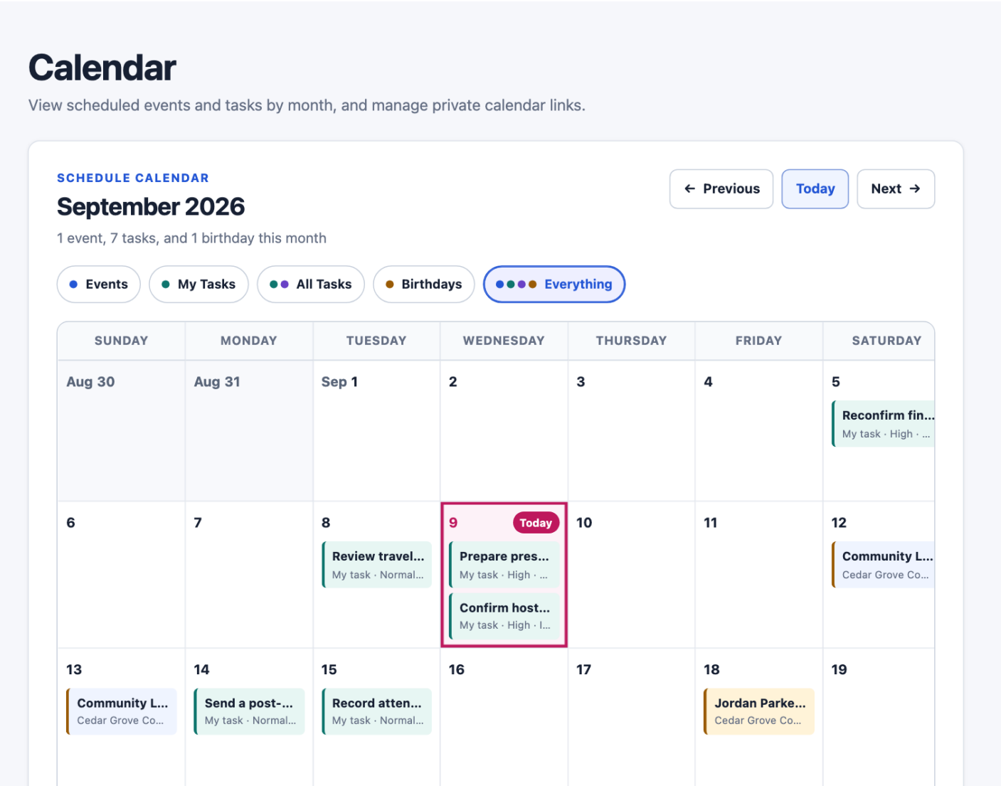
Figure 58. Browse the month calendar. Actual preview screen; fictional records.
