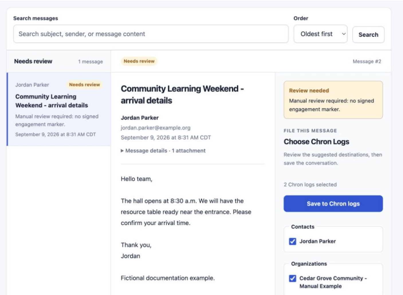
Figure 55. Read a message and choose its Chron Logs. Actual preview screen; fictional records.
