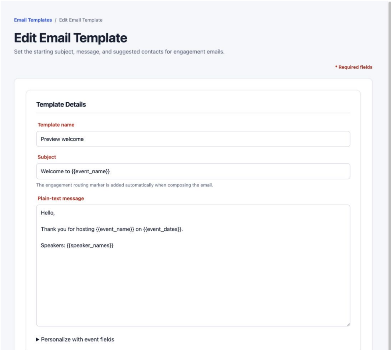
Figure 27. Add or edit reusable email text. Actual preview screen; fictional records.
