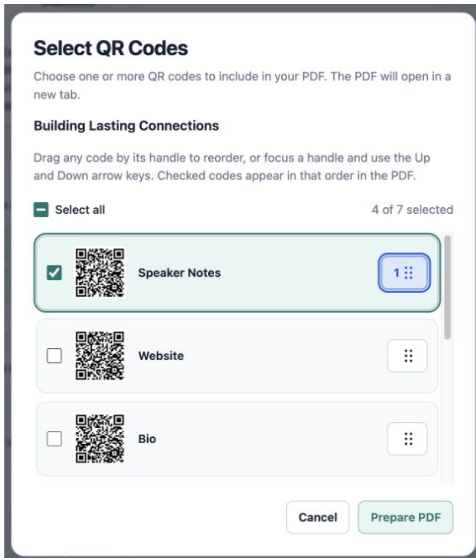
Figure 19. Select and order QR codes for a PDF. Actual preview screen; fictional records.
