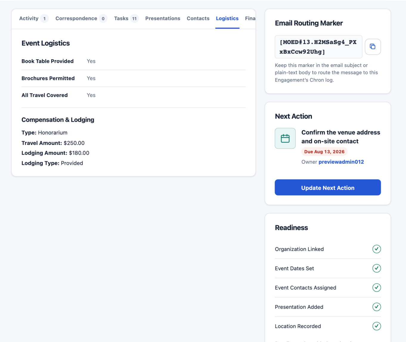
Figure 21. Review event logistics. Actual preview screen; fictional records.
