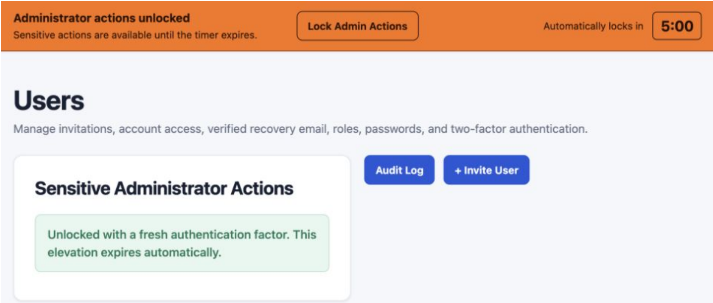
Figure 78. Unlock temporarily and lock again when finished. Actual preview screen; fictional records.
