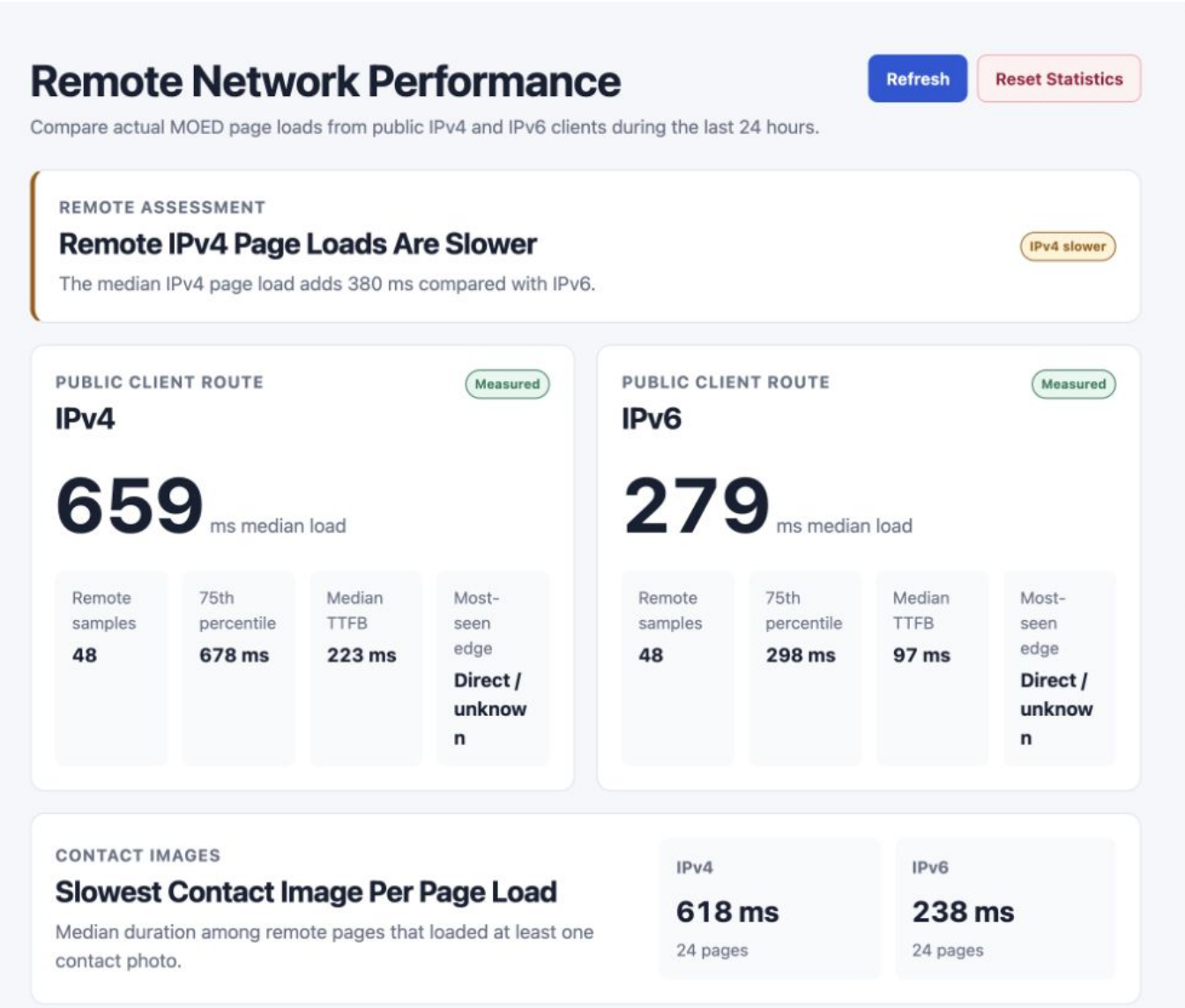
Figure 77. Compare remote IPv4 and IPv6 traffic. Actual preview screen; fictional records.
