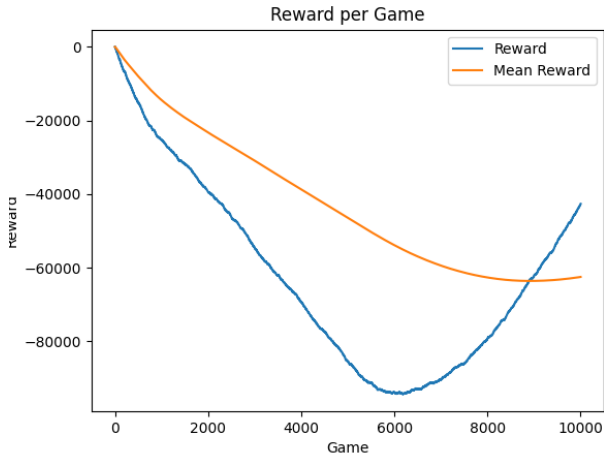
Figure 2. Reward per game and mean reward per game in training
