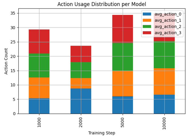
Figure 5. Average action distribution per game over 100 evaluation games
