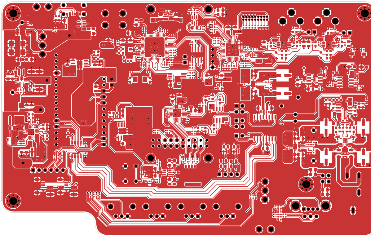
FRONT – COMPONENTS AND SIGNAL
