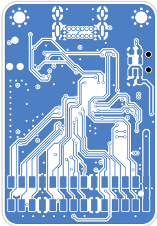
B.CU SIGNAL
