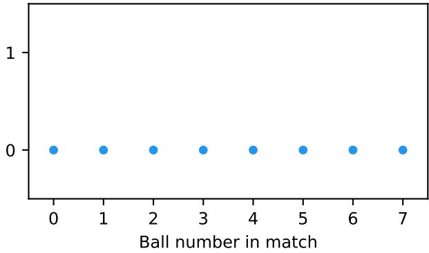
Ball-by-ball state (this match)
