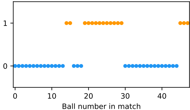
Ball-by-ball state (this match)
