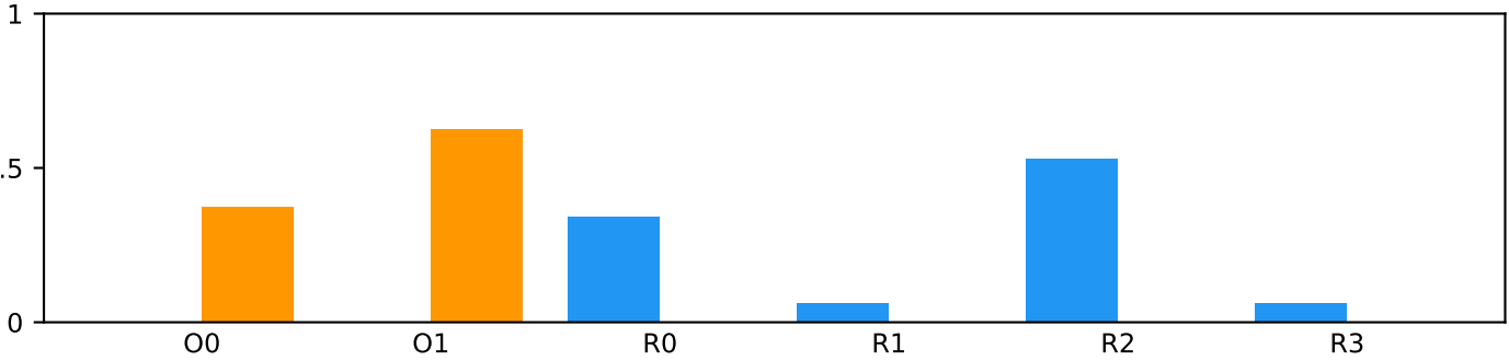
Delivery-type mix per state (see page 1 for cluster names)
