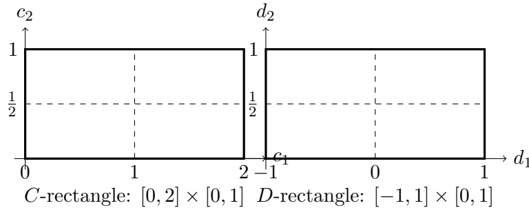
Figure 1: Equal-axis initial planar grids for C and D . Combining one rectangle from the C -grid with one rectangle from the D -grid gives a four-dimensional cell.
