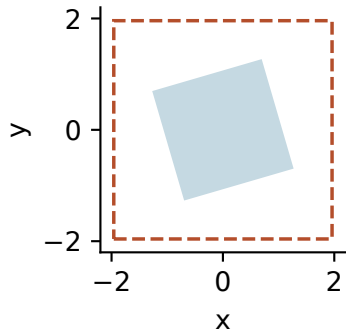
After two exact rotations
