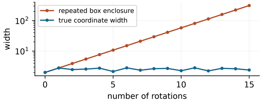
All updates use exact fractions
