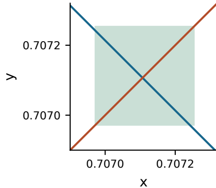
Zoom: certified Krawczyk box
