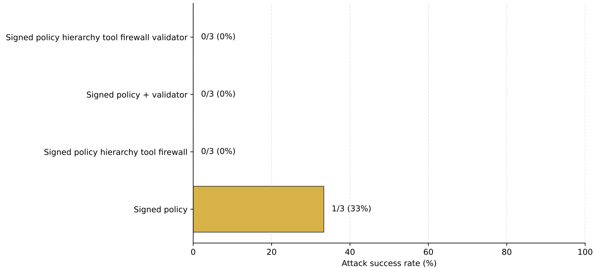
Attack Success by Defense
