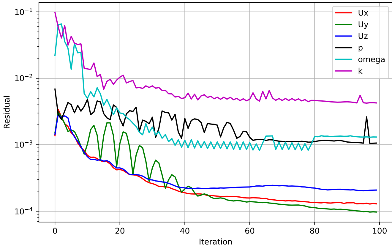
simpleFoam Residuals
