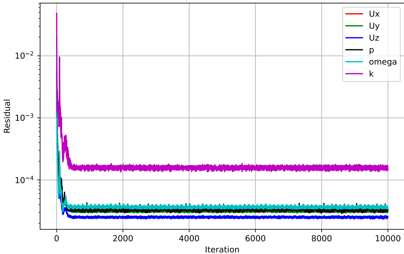
simpleFoam Residuals
