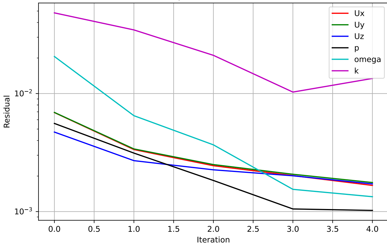
simpleFoam Residuals
