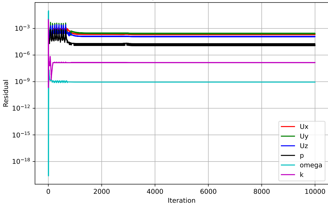
simpleFoam Residuals
