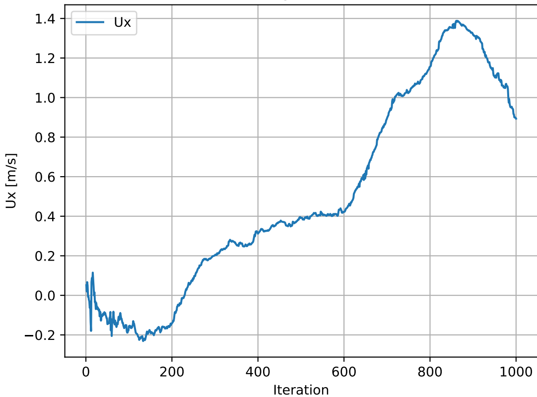
Ux convergence at outlet
