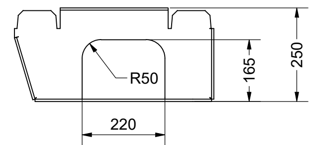
Folded Foot ( 1 : 10 )
