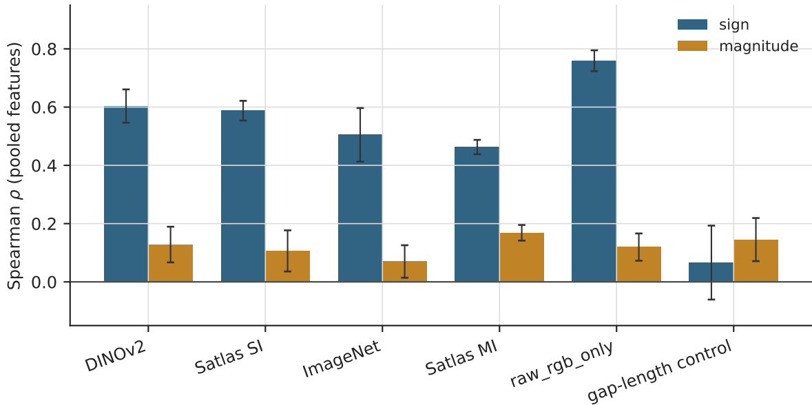
P2 screened: direction recoverable, rate is not
