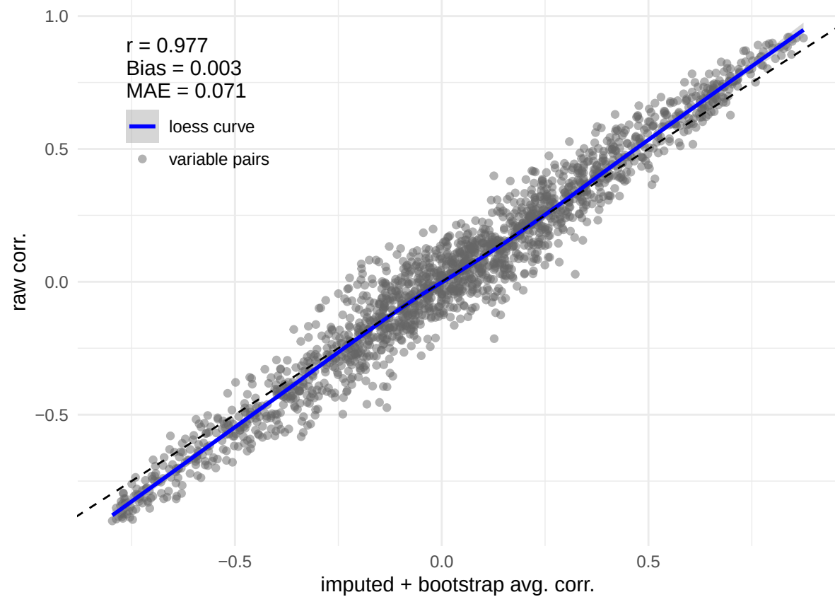
Polychoric correlations raw nemo_temp_0.5 vs. bootstrap + MICE avg.
