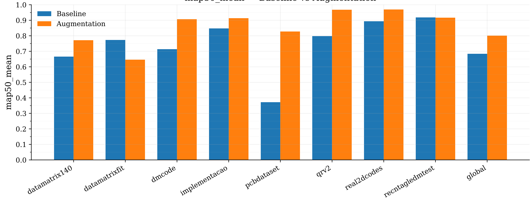
map50_mean — Baseline vs Augmentation
