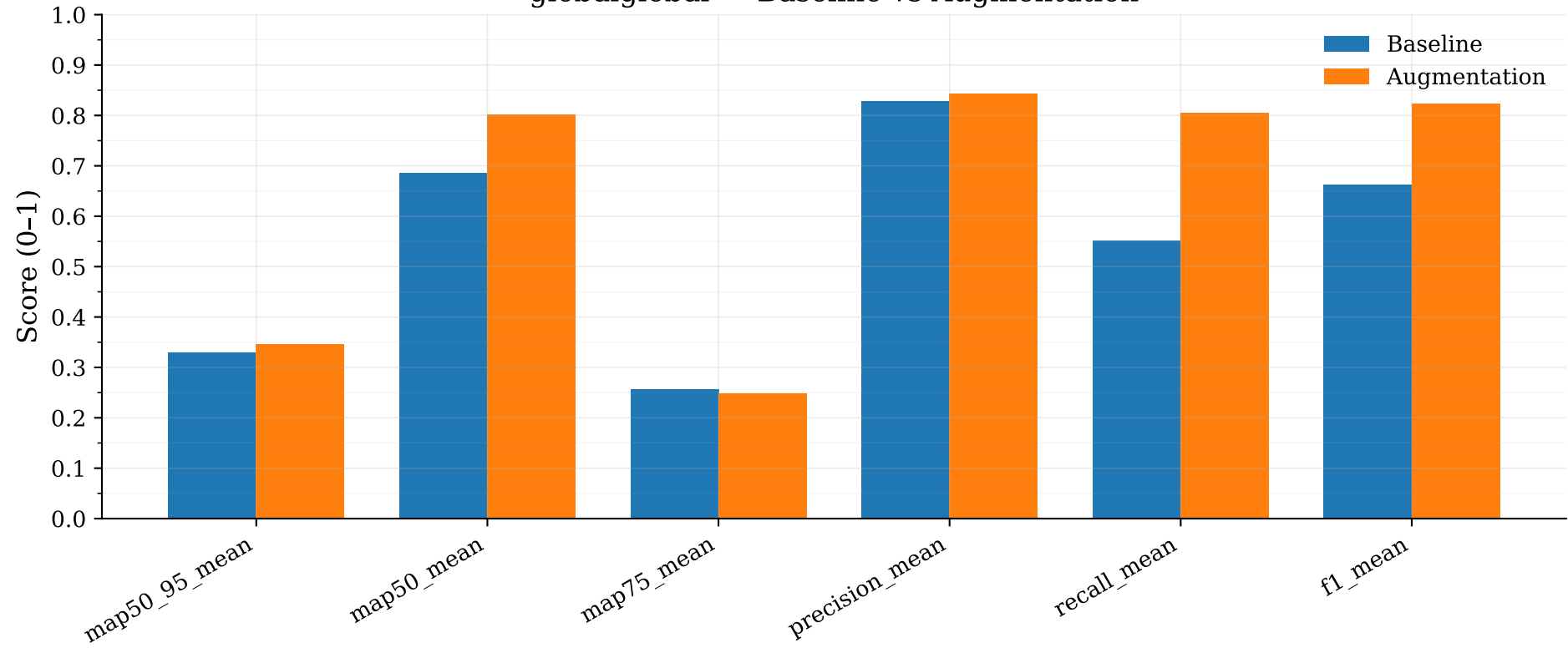
globalglobal — Baseline vs Augmentation
