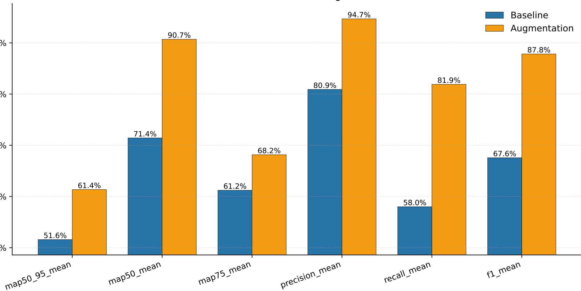
dmcode — Baseline vs Augmentation
