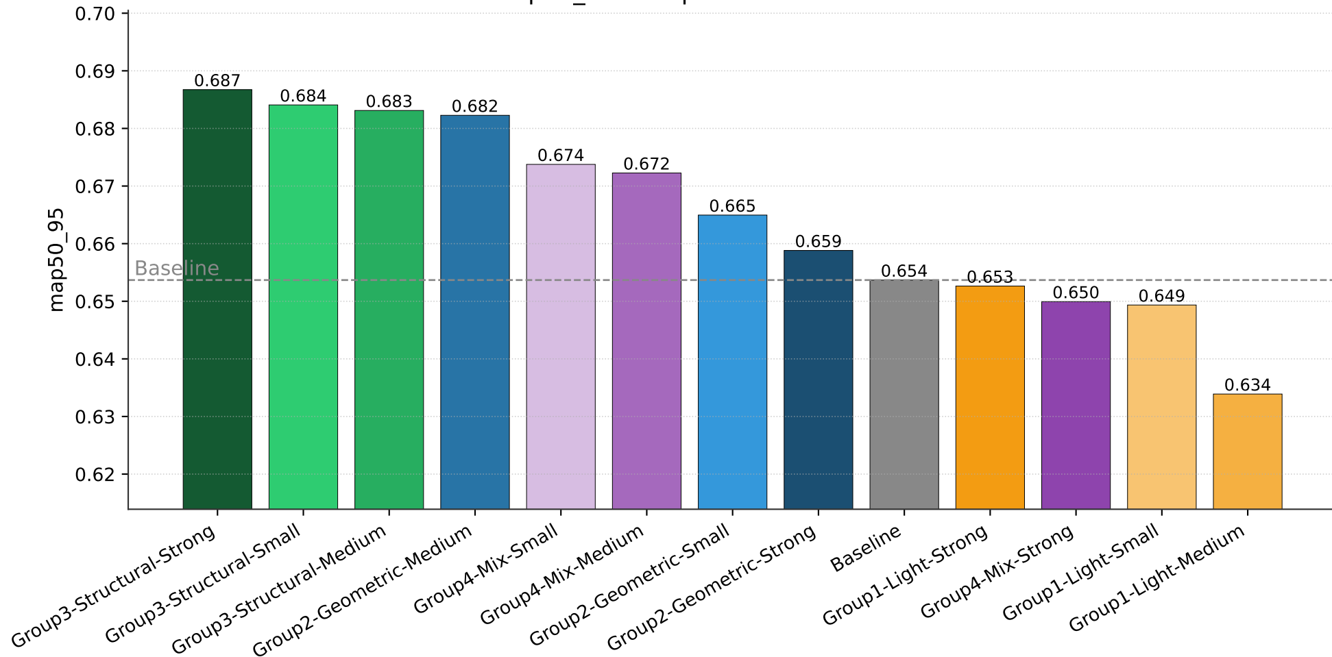
map50_95 comparison on validation set
