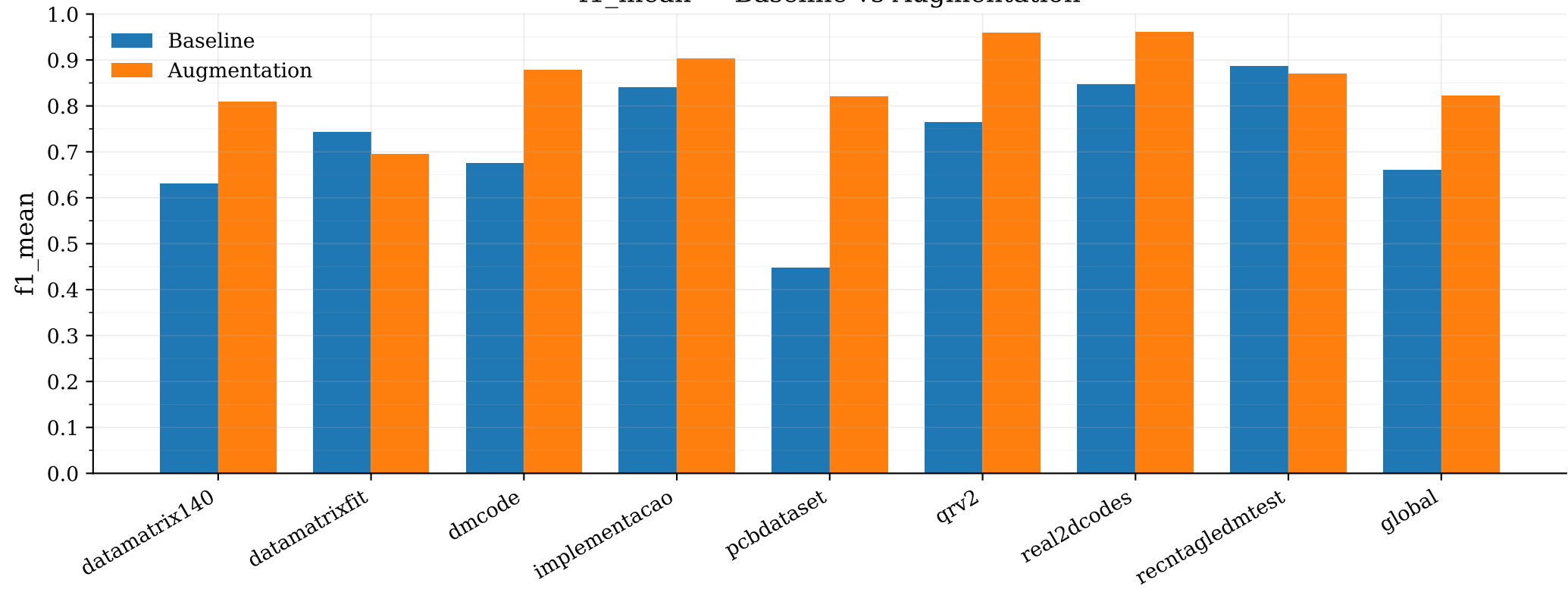
f1_mean — Baseline vs Augmentation
