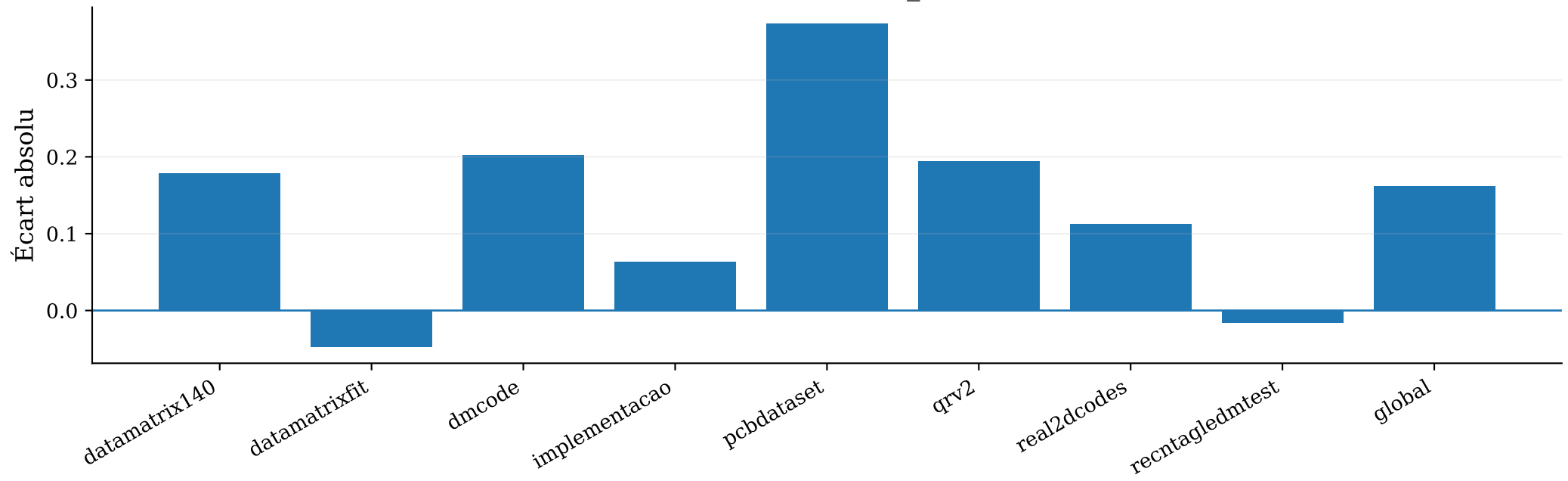
Delta (B - A) — f1_mean
