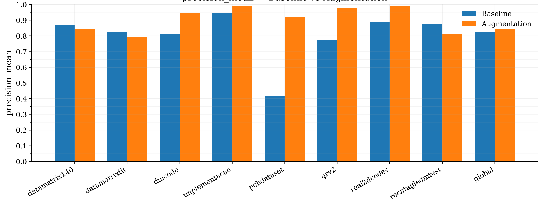
precision_mean — Baseline vs Augmentation
