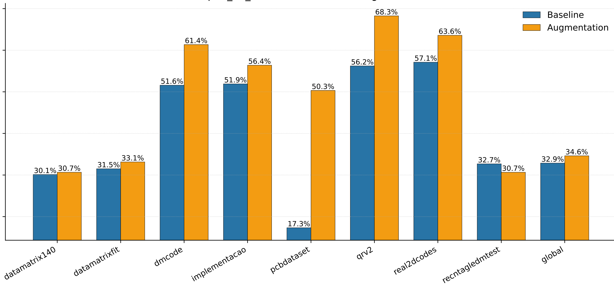
map50_95_mean — Baseline vs Augmentation
