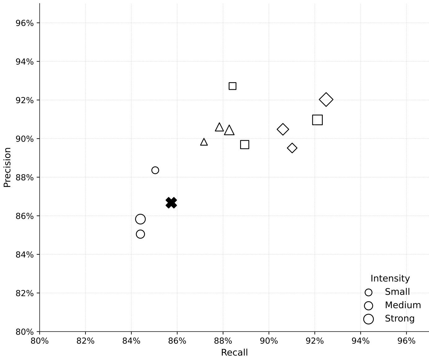
Precision vs Recall on validation set
