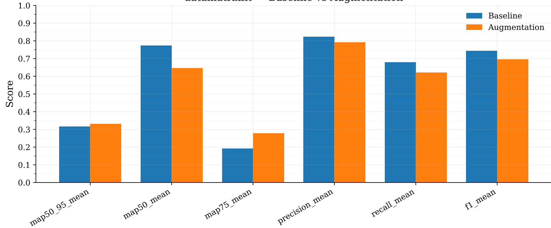
datamatrixfit — Baseline vs Augmentation
