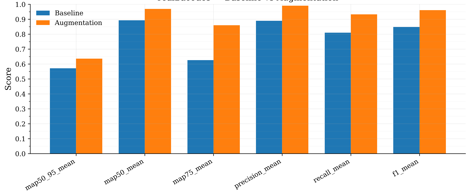
real2dcodes — Baseline vs Augmentation
