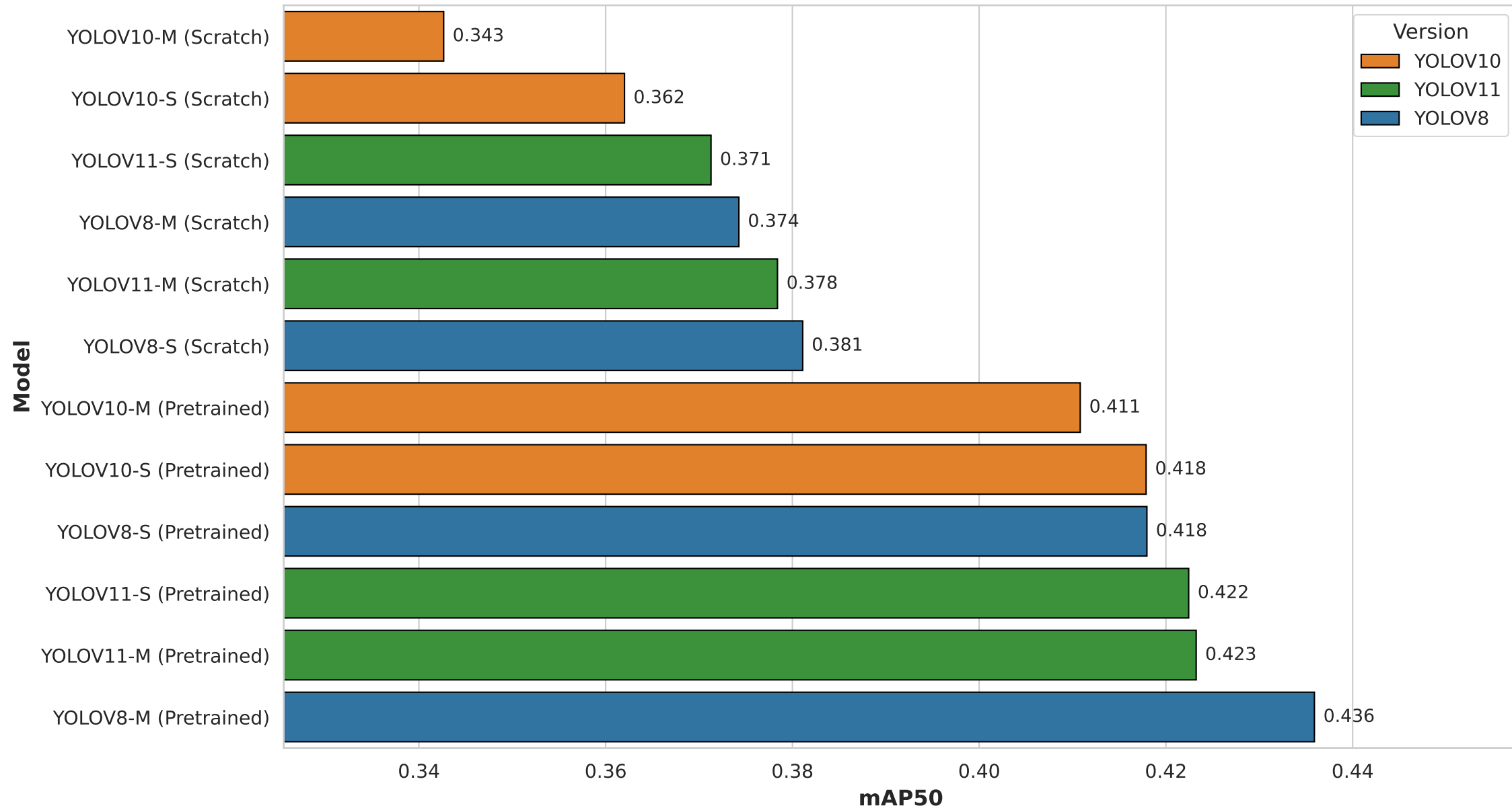
Comparison of mAP50 Across Models on validation set
