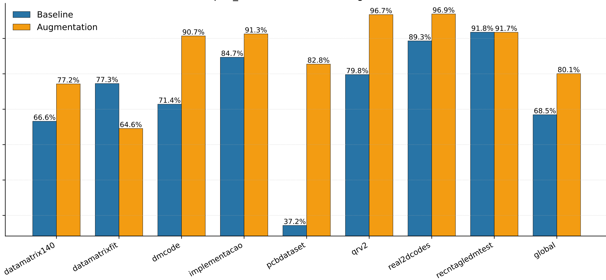
map50_mean — Baseline vs Augmentation
