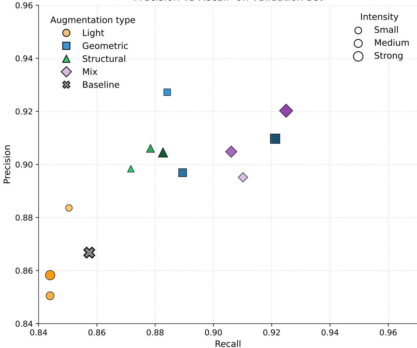
Precision vs Recall on validation set
