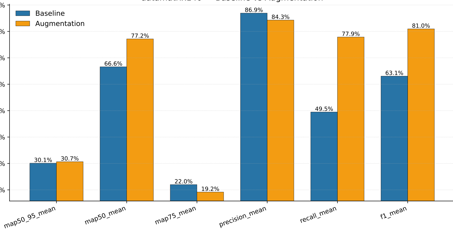
datamatrix140 — Baseline vs Augmentation
