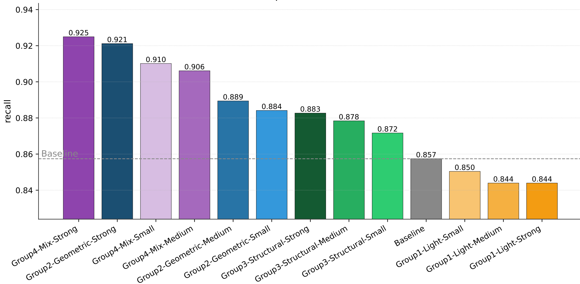
recall comparison on validation set
