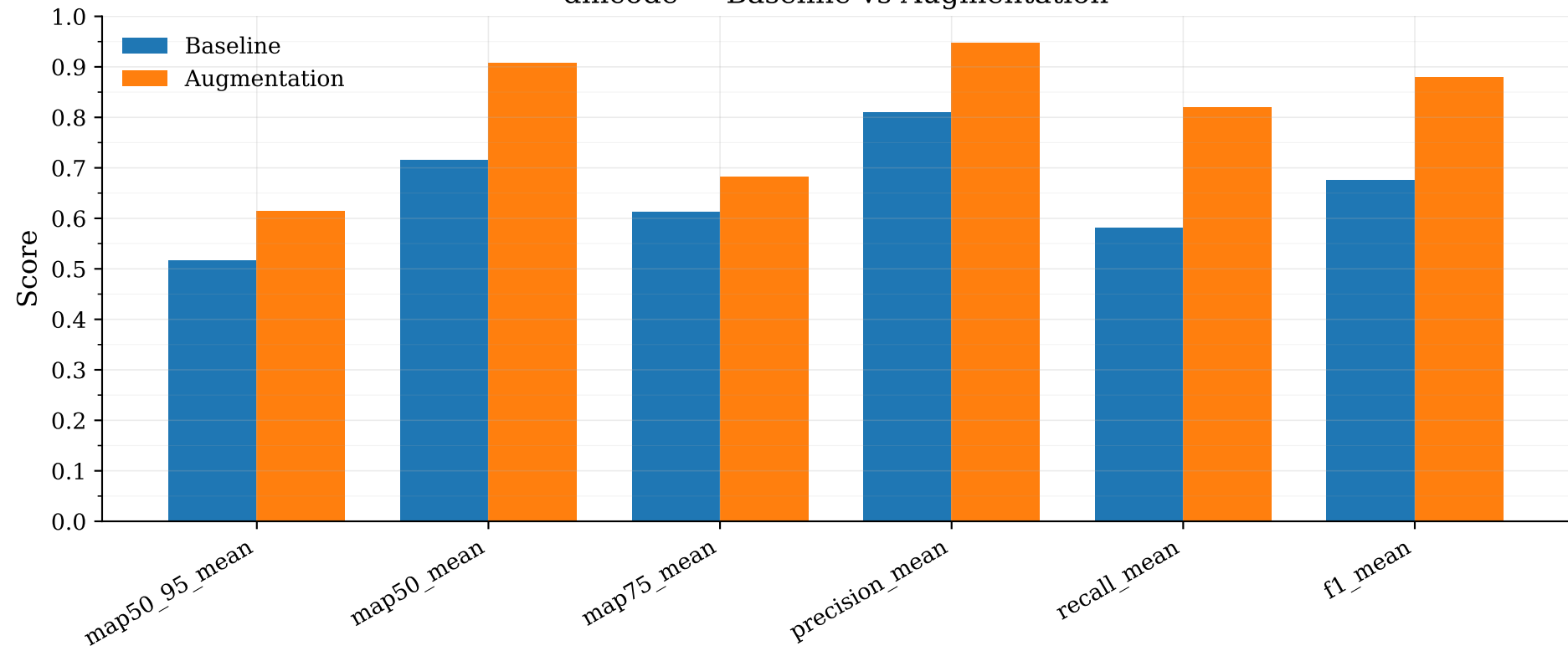
dmcode — Baseline vs Augmentation
