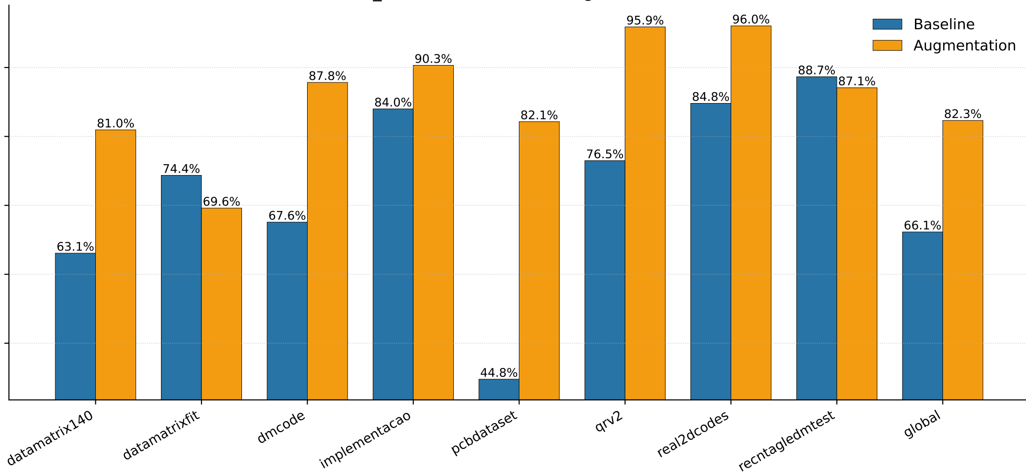
f1_mean — Baseline vs Augmentation
