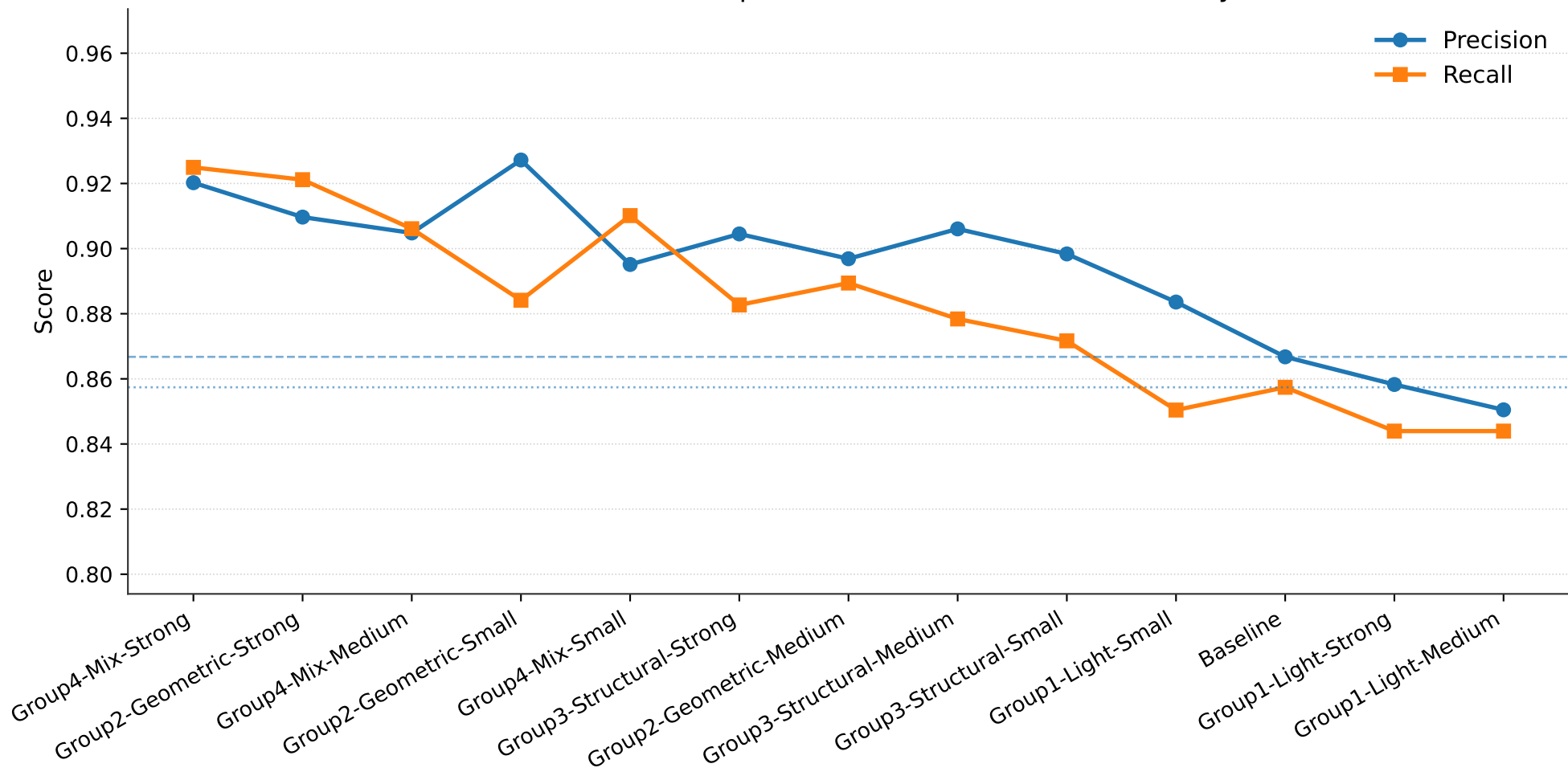
Precision & Recall comparison on validation set (sorted by f1)
