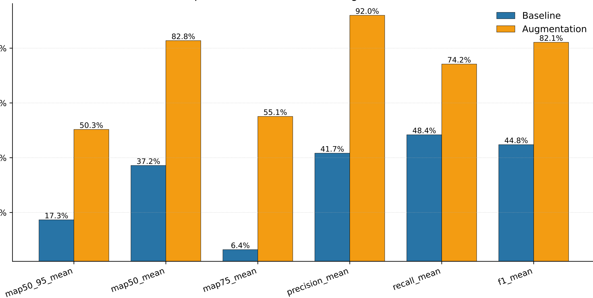
pcbdataset — Baseline vs Augmentation
