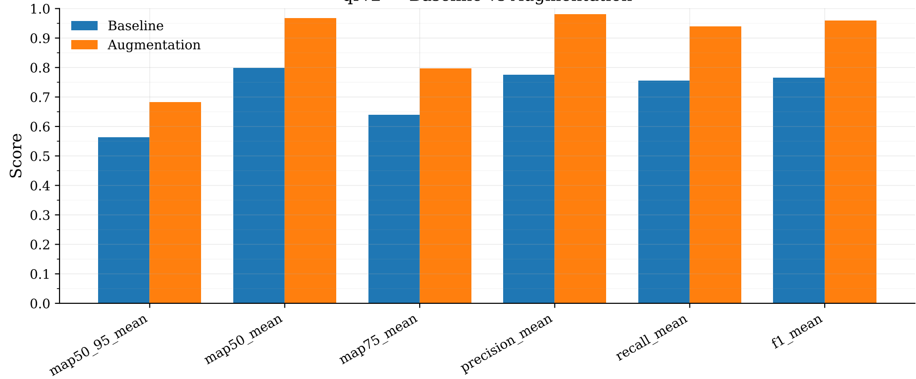
qrv2 — Baseline vs Augmentation
