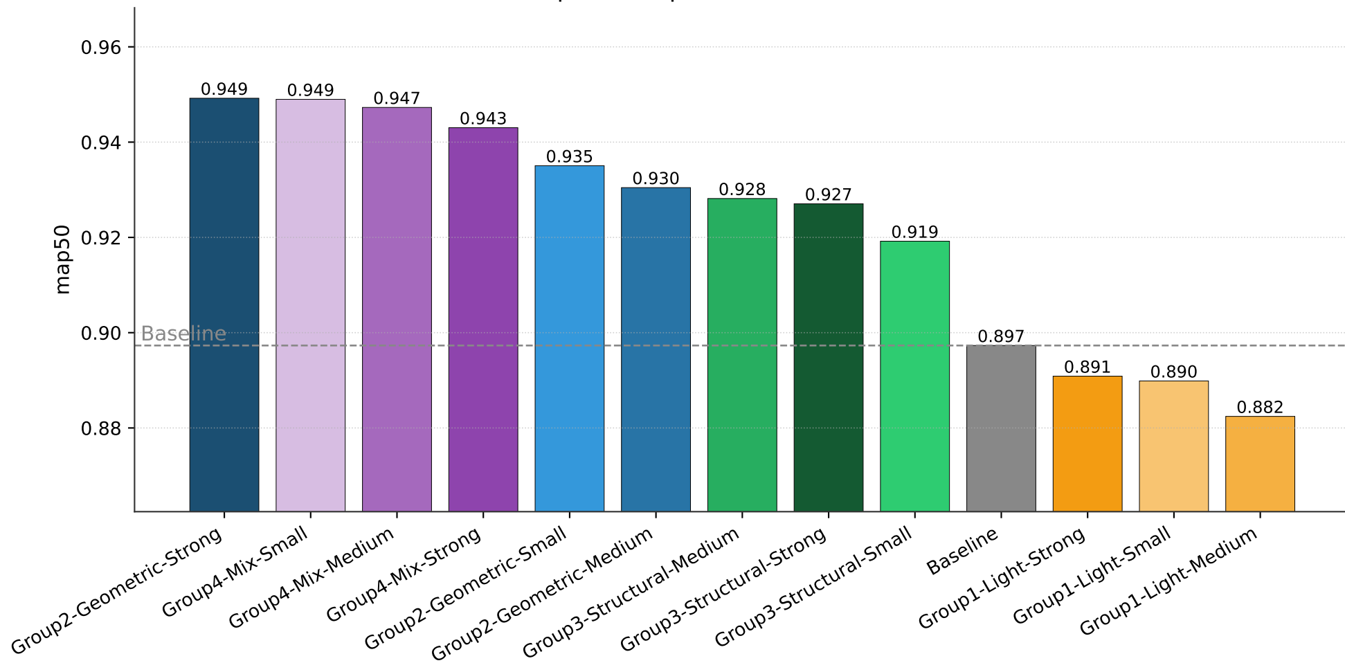
map50 comparison on validation set
