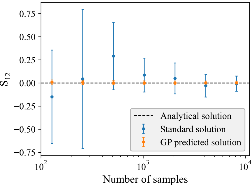
Second order effect index x_{12}
