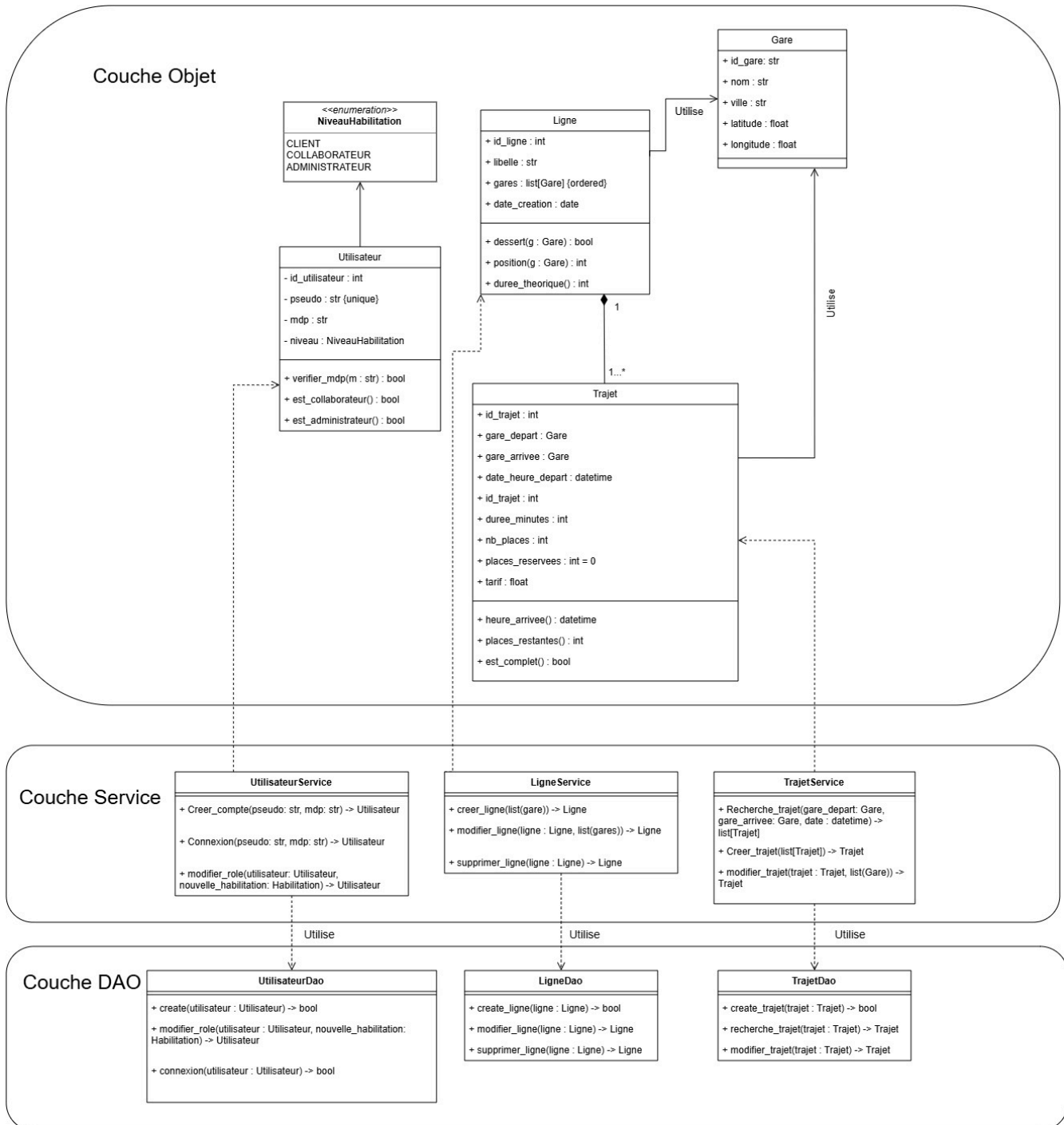
Figure 7: Classes
