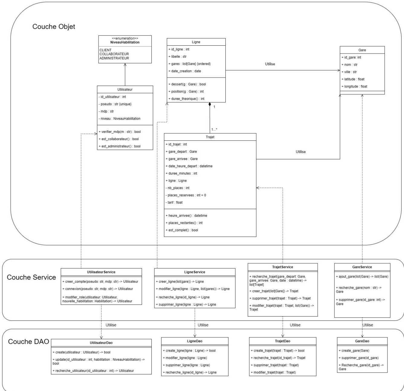
Figure 7: Classes
