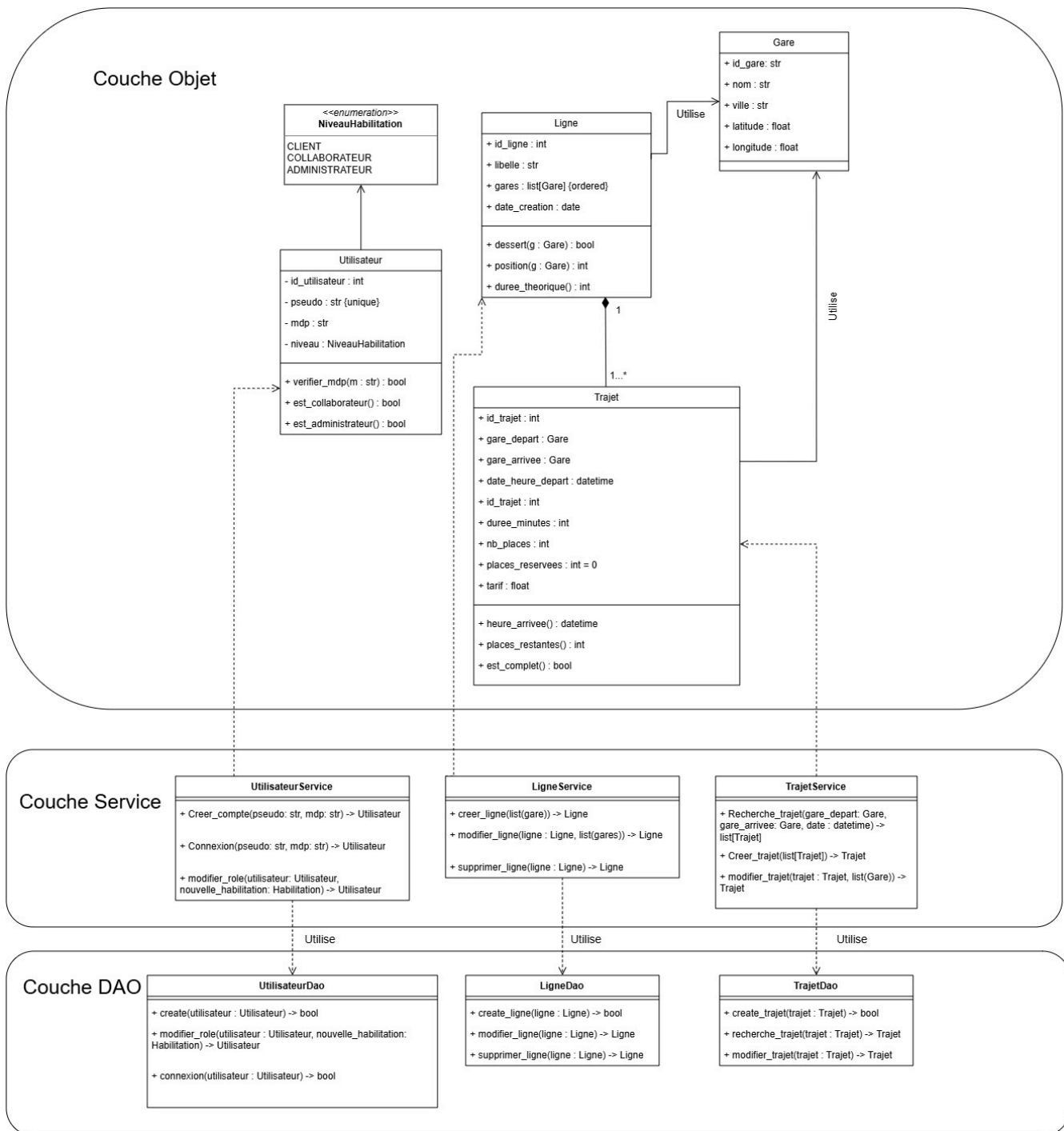
Figure 7: Classes
