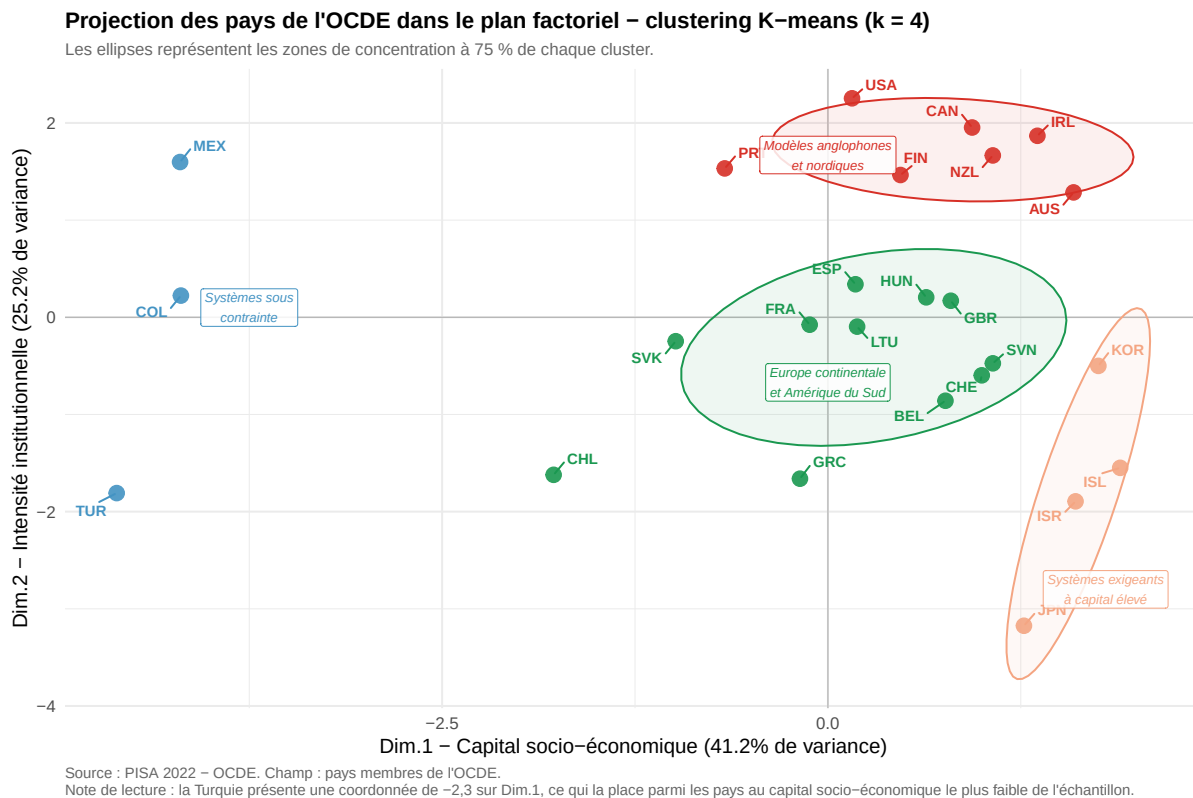
FIGURE 22 : Projection des pays — clustering K-means (k = 4)
