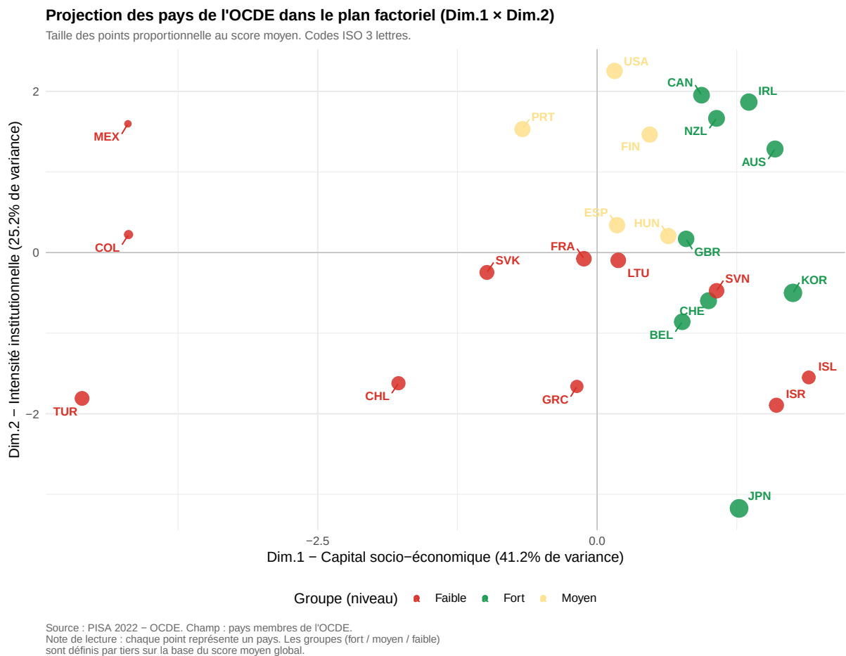
FIGURE 23 : -acp-individus
