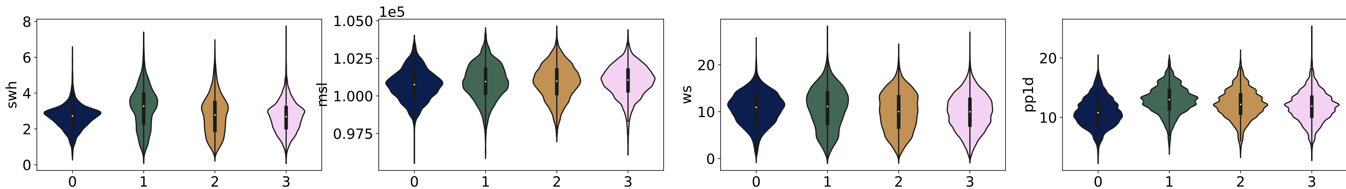
(c) Distribution of values per variable and cluster for KMeans with Euclidean distance
