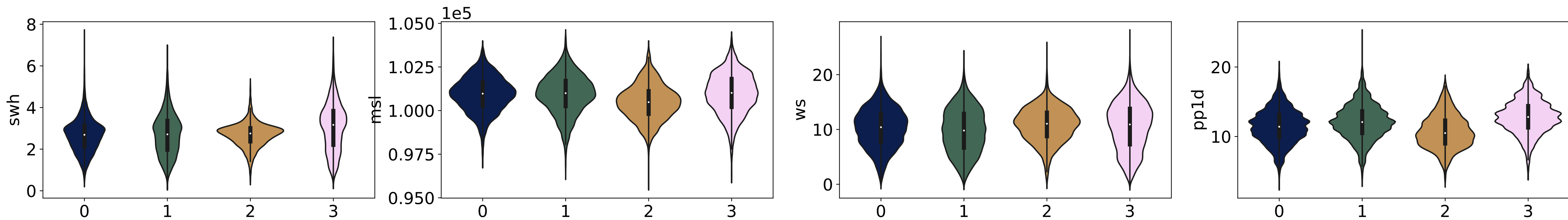
(b) Distribution of values per variable and cluster for KMeans with autoencoder and PCA
