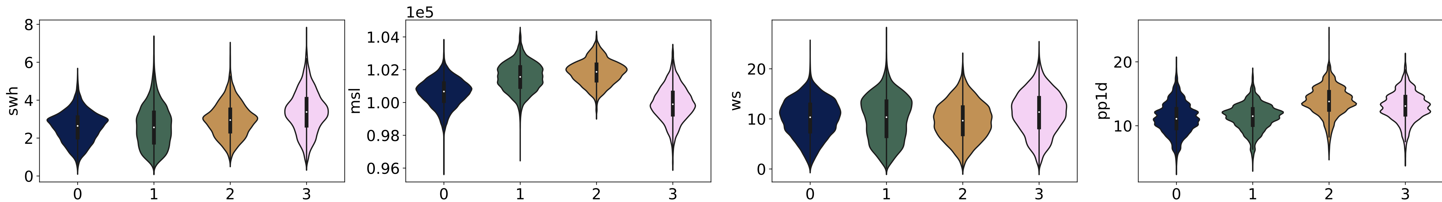
(a) Distribution of values per variable and cluster for KMeans with DTW measure
