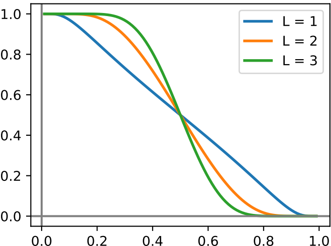
Boyd function
